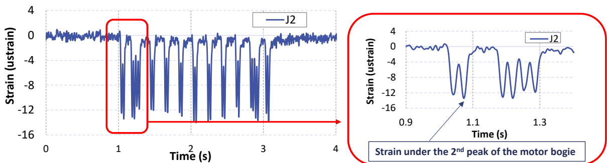
Figure 11. Vertical strain signal (and zooming) recorded on Section 2 (with UGM layer) with J2 strain gauge, V=160 km/h
