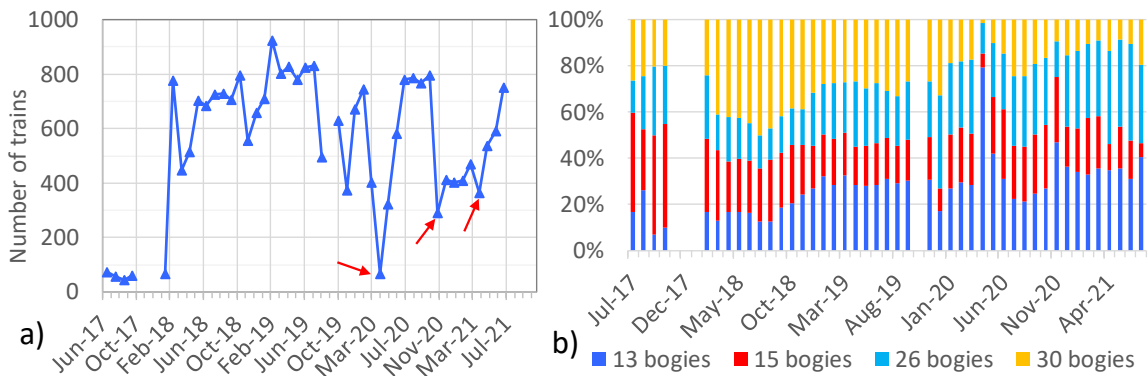
Figure 7. Number on train (a) and distribution of type of train (b) operating, each month, on Section 4 (with bituminous sub-layer)
