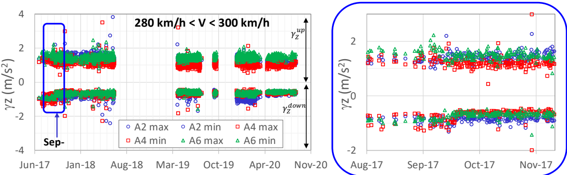
Figure 19. Acceleration under the signal second peak recorded by accelerometers A2, A4 and A6 (located under the outer rail) on Section 1 (with bituminous sub-layer) from July 2017 to September 2020 for 26 bogie-trains and a speed within the range of 280-300 km/h, as a function of time, and zoomed view
