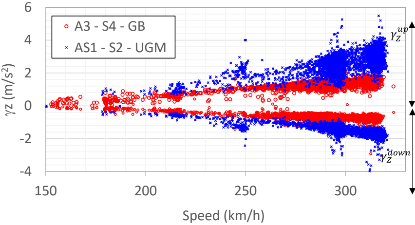
Figure 25. Comparison of positive and negative vertical acceleration peaks, under the signal second peak, recorded on Section 2 (with granular sub-layer) and Section 4 (with bituminous sub-layer) accelerometer AS1 and A3 (both located below the outer rail), respectively, during the commercial phase from July 2017 to July 2021 for 26 bogie-trains as a function of speed
