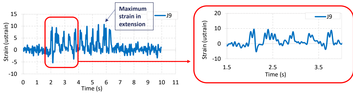
Figure 12. Transverse strain signal (and zooming) recorded on Section 4 (with GB layer) with J9 strain gauge, V=165 km/h
