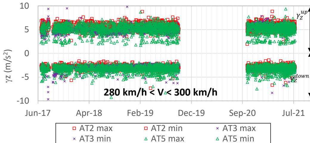
Figure 23. Acceleration under the signal second peak recorded on Section 2 (with granular sub-layer), from accelerometers AT2, AT3 and AT5, located at the top of the sleepers, from July 2017 to July 2021 for 26 bogie-trains and a speed within the range of 280-300 km/h, as a function of time
