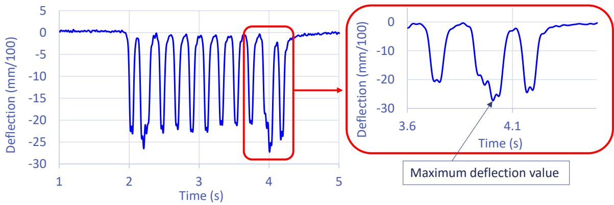
Figure 10. Deflection signal recorded on Section 2 (with UGM layer) with sensor 2, V=320 km/h
