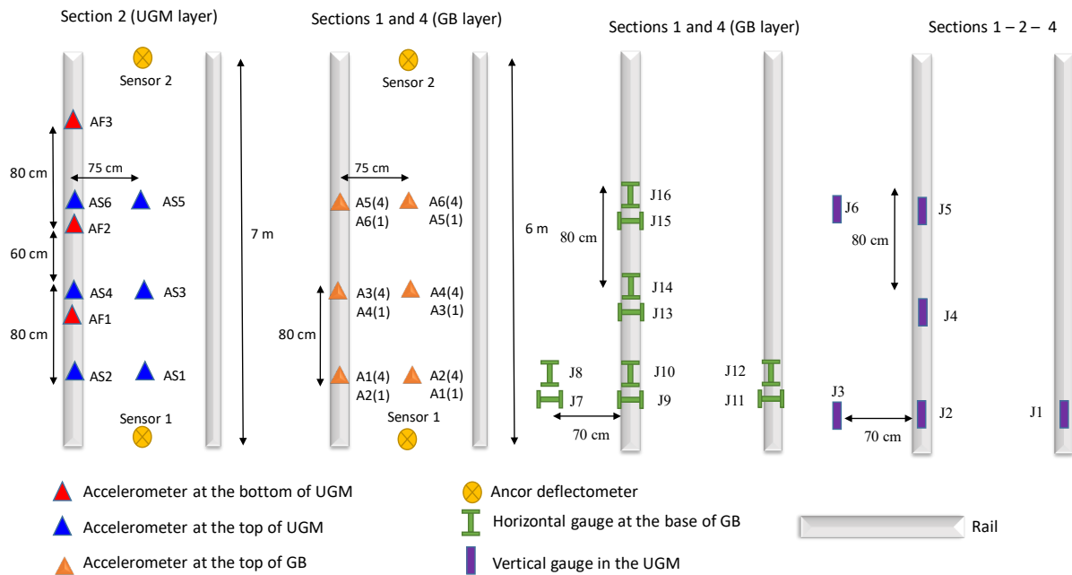
Figure 3. Layout of the instrumentation for accelerometers, displacement sensors, vertical and horizontal strain gauges
