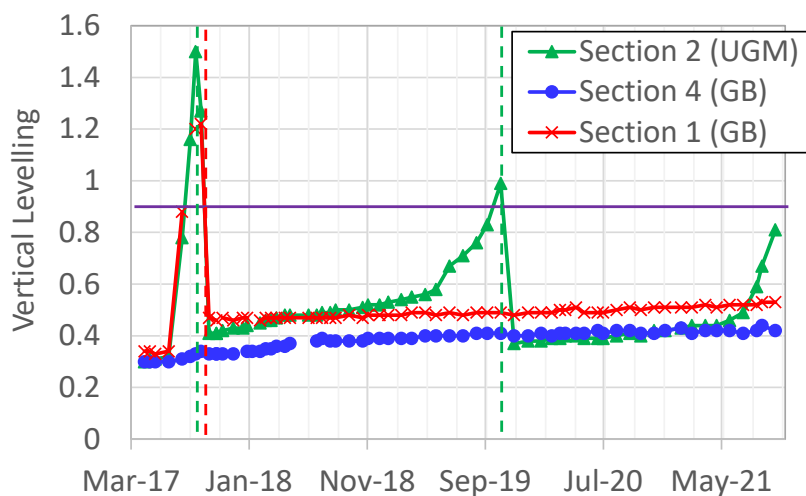
Figure 26. Vertical levelling measured on distances of 200 meters including Sections 2, 1 and 4
