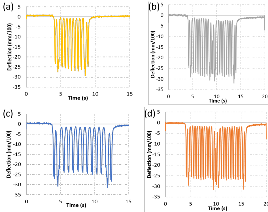
Figure 6. Example of temporal deflection signals from both single and double trains with (a) 13 bogies, (b) 26 bogies, (c) 15 bogies and (d) 30 bogies, running Section 4 on opening day
