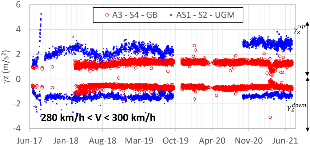
Figure 24. Comparison of positive and negative vertical acceleration peaks, under the signal second peak, recorded on Section 2 (with granular sub-layer) and Section 4 (with bituminous sub-layer) accelerometer AS1 and A3 (both located below the outer rail), respectively, during the commercial phase from July 2017 to July 2021 for 26 bogie-trains and a speed within the range of 280-300 km/h
