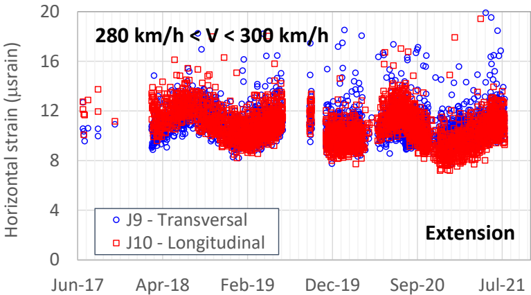
Figure 15. Maximum values for transverse and longitudinal strain from gauge J9 and gauge J10, respectively, recorded for 26 bogie-trains on Section 4 (with bituminous sub-layer) as a function of time from July 2017 to July 2021, for a train speed ranging from 280 to 300 km/h
