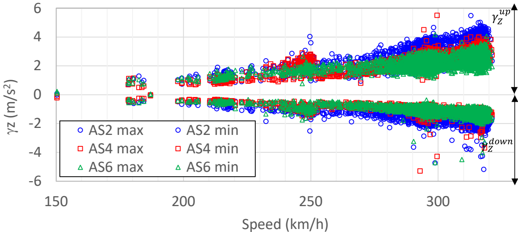
Figure 20. Acceleration under the signal second peak recorded on Section 2 (with granular sub-layer) by accelerometers AS2, AS4 and AS6 at the surface of the UGM layer (located below the outer rail) from July 2017 to July 2021 for 26-bogie trains as a function of speed
