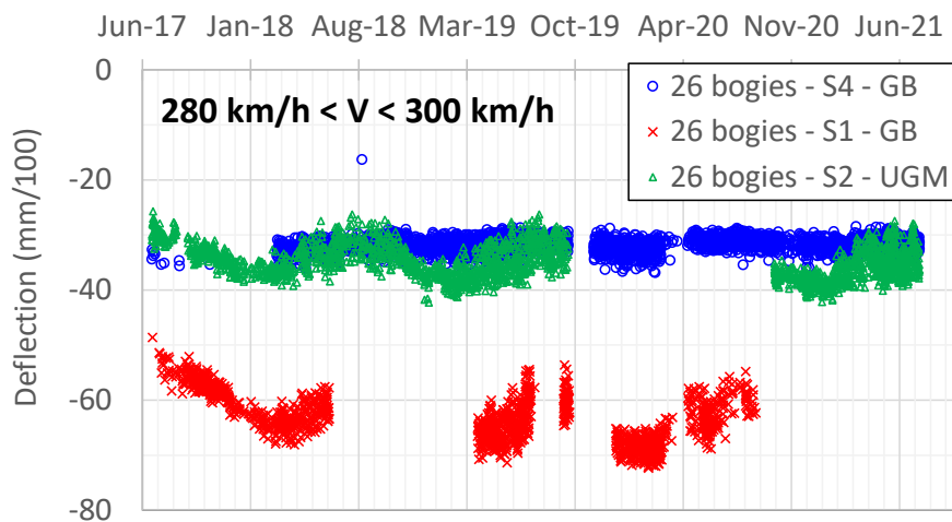
Figure 13. Comparison between the maximum deflection values measured on Section 2 (with granular sub-layer) and Sections 4 and 1 (with bituminous sub-layer) from July 2017 to July 2021, for trains with 26 bogies, for a train speed ranging between 280 and 300 km/h
