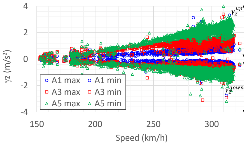
Figure 16. Acceleration under the signal second peak recorded for 26 bogie-trains on Section 4 (with bituminous sub-layer) by accelerometers A1, A3 and A5 (located below the outer rail) from July 2017 to July 2021, as a function of speed
