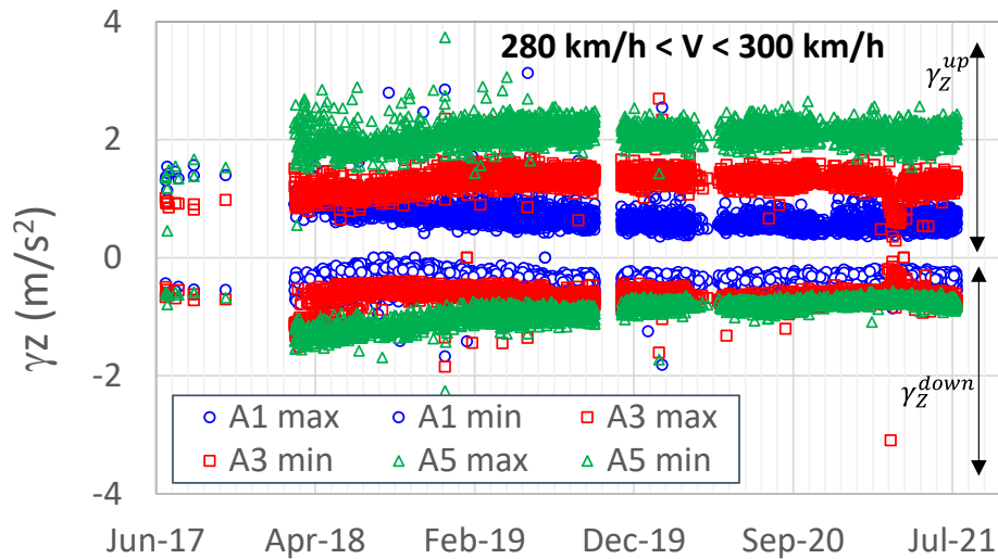
Figure 17. Acceleration under the signal second peak recorded on Section 4 (with bituminous sub-layer) by accelerometers A1, A3 and A5 (located under the outer rail) from July 2017 to July 2021 for 26 bogie-trains and a speed within the range of 280-300 km/h as a function of time
