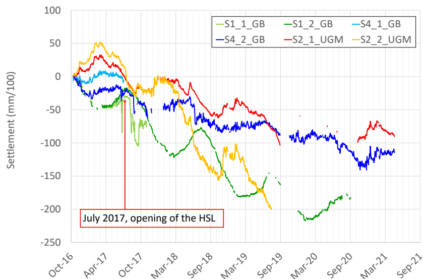
Figure 5. Evolution of track settlement on Sections 1, 2 and 4 during four years
