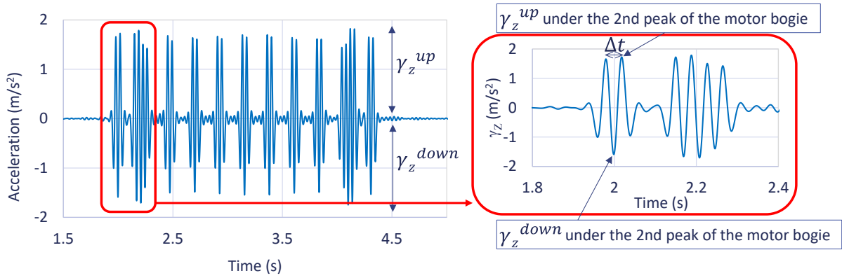
Figure 9. Vertical acceleration signal after filtering (and zooming) recorded on Section 2 (with UGM layer) with AS1 accelerometer, V=295 km/h
