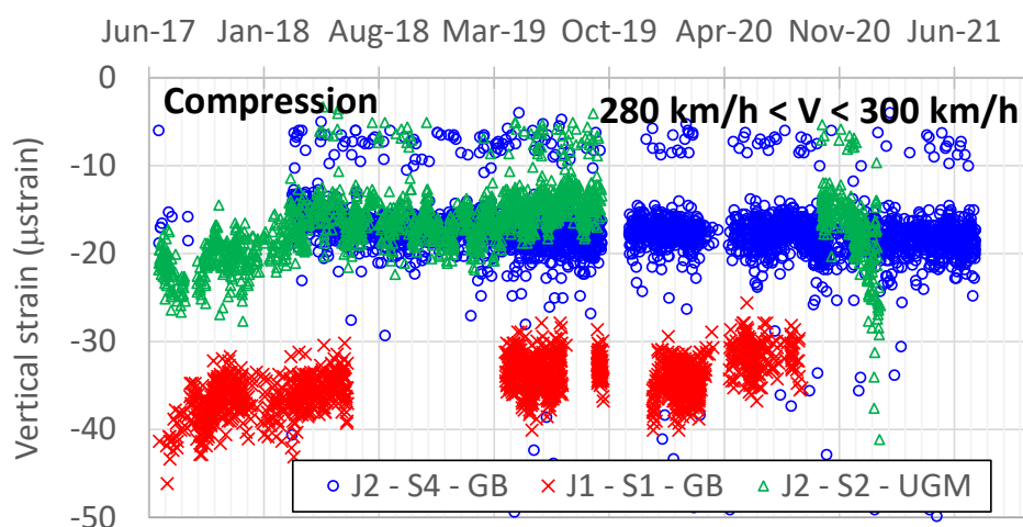
Figure 14. Comparison between the maximum vertical strain values in compression mode measured on Section 2 (with granular sub-layer) and Sections 4 and 1 (with bituminous sub-layer) from July 2017 to July 2021 for 26 bogie-trains and a speed ranging between 280 and 300 km/h
