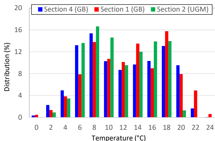
Figure 4. Histogram of the temperature distribution over 4 years (2017-2020) at the bottom of the ballast layer, for the three instrumented sections
