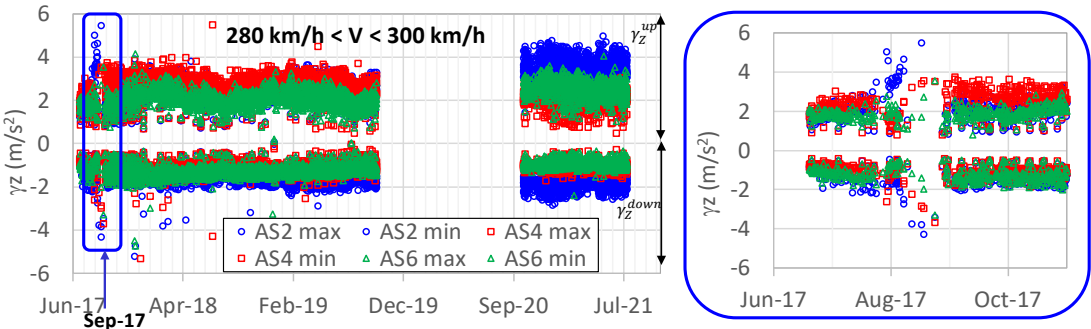
Figure 21. Acceleration under the signal second peak recorded on Section 2 (with granular sub-layer) by accelerometers AS2, AS4 and AS6 at the surface of the UGM layer (located below the outer rail) from July 2017 to July 2021 for 26-bogie trains as a function of time, and zoomed view
