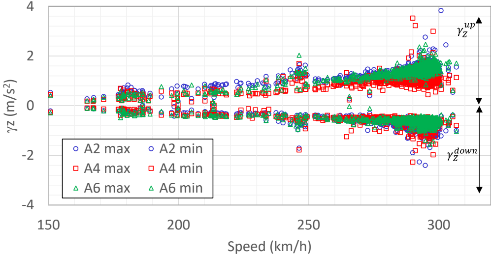
Figure 18. Acceleration under the signal second peak recorded by accelerometers A2, A4 and A6 (located under the outer rail) on Section 1 (with bituminous sub-layer) for 26 bogie-trains from July 2017 to September 2020, as a function of speed
