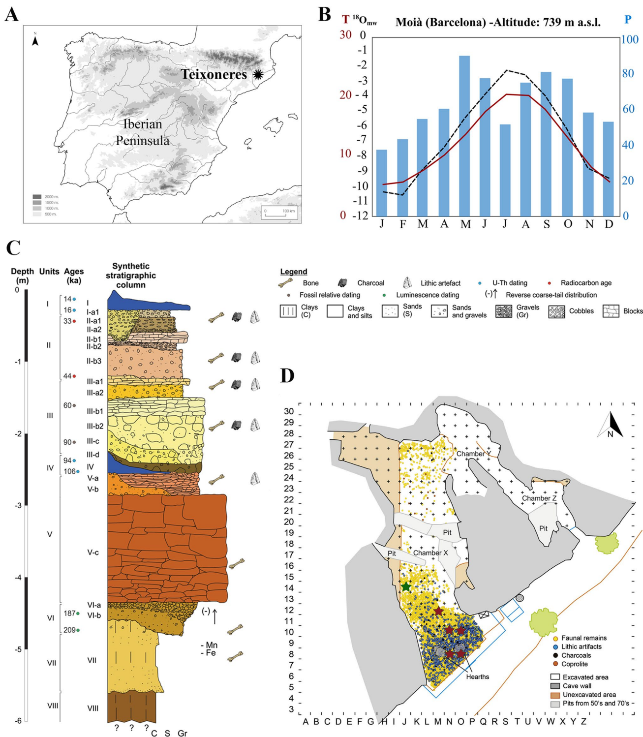
Fig. 1 A Location of the Teixoneres Cave in Iberia; B current monthly temperatures (continuous line; T; in °C) and precipitations (bars; P; in mm) (Climate-data.org) and present-day oxygen isotope composition of meteoric waters (dash black; \delta^{18}O_{mw} 2017) of Moia; C synthetic stratigraphic sequence of chamber X in Teixoneres Cave, modified from Zilio et al. (2021); U-Th series (Tissoux et al. 2006)
