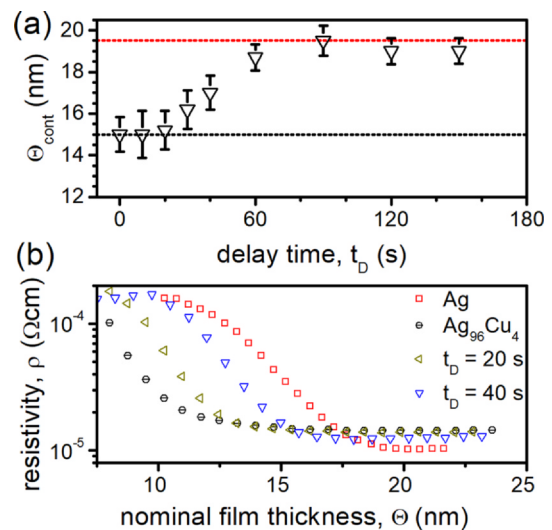
Fig. 8. (a) Evolution of the continuous film formation thickness \Theta_{cont} of Ag_{100-x}Cu_x films vs. delay time t_D of the Cu deposition. Error bars correspond to the standard error from determining \Theta_{cont} from resistivity \rho vs. nominal thickness \Theta plots. Horizontal dotted lines mark \Theta_{cont} for Ag (red) and co-deposited Ag_{96}Cu_4 film (black). (b) Evolution of \rho vs. \Theta for Ag, Ag_{96}Cu_4 co-deposition (also presented in Fig. 1) and Ag_{100-x}Cu_x with delay times t_D = 20 s and 40 s. (For interpretation of the references to colour in this figure legend, the reader is referred to the web version of this article.)
