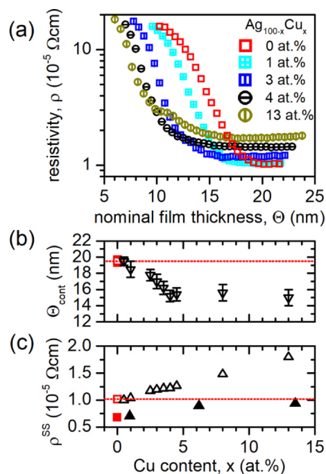
Fig. 1. (a) Resistivity ( \rho ) vs. nominal thickness ( \Theta ) curves extracted from in situ , real-time spectroscopic ellipsometry measurements, of magnetron sputter-deposited Ag and Ag 100-x Cu x layers on SiO 2 /Si substrates with increasing Cu content x in the film. Evolution of (b) the continuous film formation thickness \Theta_{cont} , and (c) steady-state resistivity \rho^{SS} of Ag 100-x Cu x films vs. Cu content x in the film (hollow symbols). Room-temperature resistivity values of continuous Ag 100-x Cu x layers determined from ex situ four-point-probe measurements are also plotted in (c) (full symbols). Error bars correspond to the standard error from determining \Theta_{cont} from resistivity vs. thickness plots presented in (a). The horizontal dotted lines represent the respective reference values for pure Ag films.
