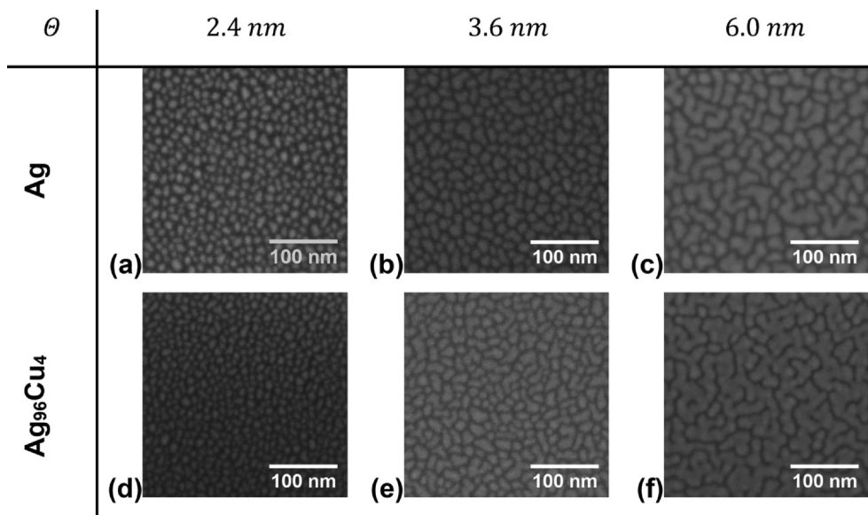
Fig. 5. Scanning electron microscopy images of Ag ((a), (b), (c)) and Ag 96 Cu 4 films ((d), (e), (f)) with nominal thicknesses 2.4 nm ((a),(d)), 3.6 nm ((b), (e)), and 6.0 nm ((c), (f)).
