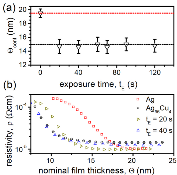
Fig. 7. (a) Evolution of the continuous film formation thickness \Theta_{cont} of Ag_{100-x}Cu_x films vs. exposure time t_E to Cu. Error bars correspond to the standard error from determining \Theta_{cont} from resistivity \rho vs. nominal film thickness \Theta plots. Horizontal dotted lines mark \Theta_{cont} for Ag (red) and co-deposited Ag_{96}Cu_4 film (black). (b) Evolution of \rho vs. \Theta for Ag, Ag_{96}Cu_4 co-deposition (also presented in Fig. 1) and Ag_{100-x}Cu_x with exposure times t_E = 20 s and 40 s. (For interpretation of the references to colour in this figure legend, the reader is referred to the web version of this article.)
