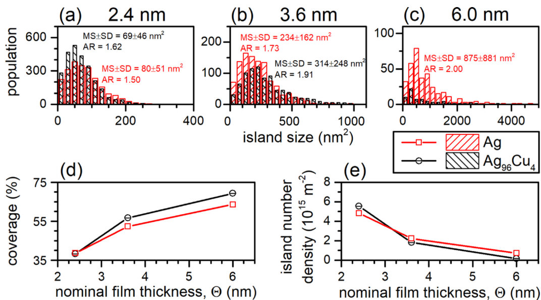
Fig. 6. (a)–(c) Island/cluster size distributions for discontinuous Ag and Ag 96 Cu 4 films with nominal thicknesses of (a) 2.4 nm, (b) 3.6 nm and (c) 6.0 nm. Mean islands size ( MS ), standard deviation ( SD ), and mean aspect ratio ( AR ) of islands are given for films that consist mainly of isolated islands. In (c) island sizes >5000 nm 2 are not presented for Ag (one island with 10000 nm 2 ) and Ag 96 Cu 4 films (eight islands ranging 7000 to 22000 nm 2 , one island with 180000 nm 2 ). Evolution of (d) coverage and (e) island number density vs. nominal film thickness of Ag and Ag 96 Cu 4 films. Data obtained by analyzing scanning electron micrographs with an area of 850 × 550 nm 2 .
