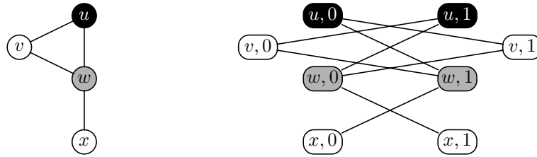
■ Figure 3 A graph (on the left) and its Kronecker cover (on the right).
