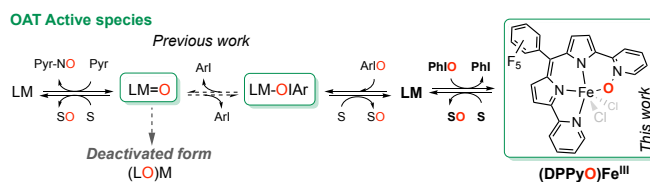
Scheme 1. Generation of relevant species involved in OAT reactions with iodosylarene and pyridine N-oxide oxidants.
