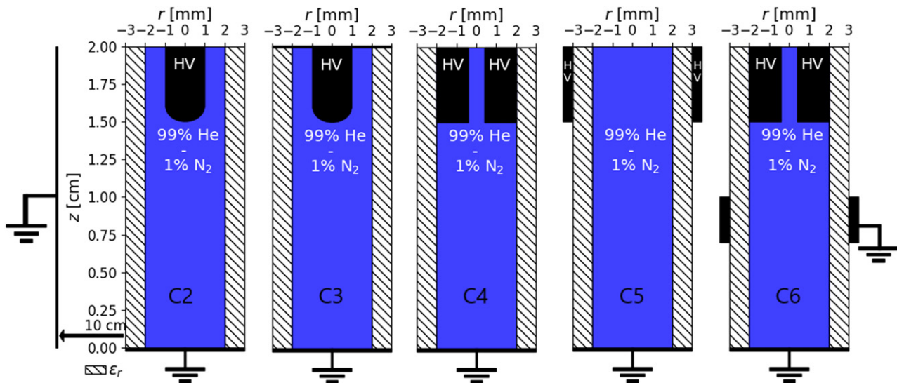
Figure 13. Side view schematics of discharge setups with different electrode geometries. From left to right: cases 2 to 6 listed in the text.
