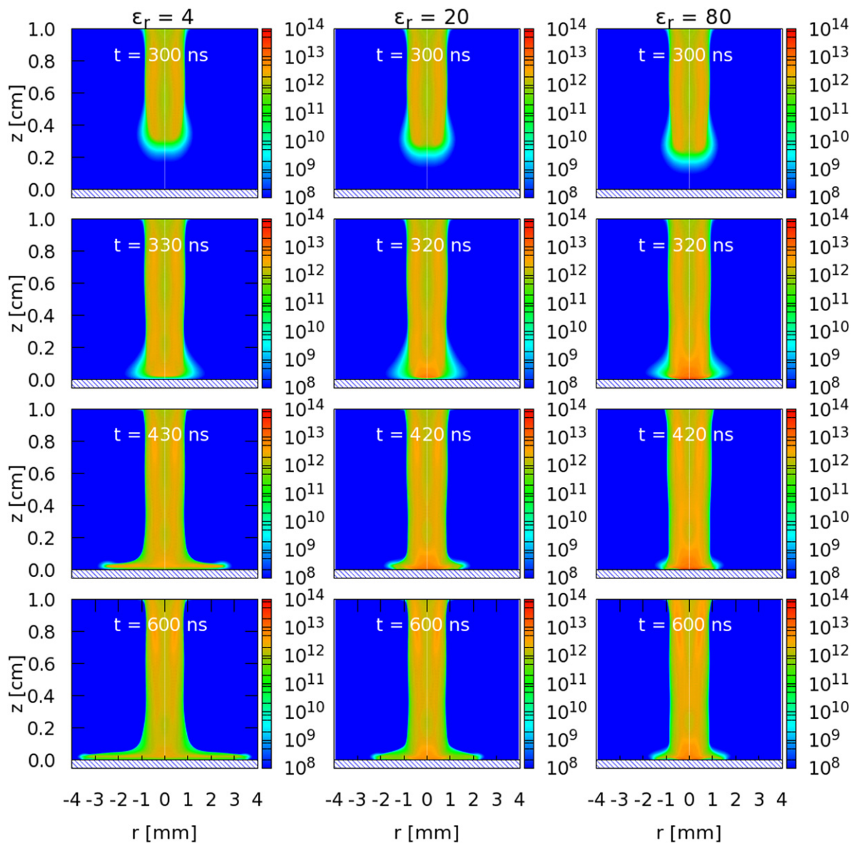
Figure 19. Cross section of spatial distribution of electron density in the plasma plume, from simulations, for V_p = 6 kV. From left to right: \epsilon_r = 4, 20 and 80 . From top to bottom: discharge propagation in the plasma plume, discharge impact, radial spreading 100 ns after impact and immediately before end of pulse. Figure reprinted by permission from Springer Nature Customer Service Centre GmbH: Springer, Plasma Chemistry and Plasma Processing (2020) 40 661–683 Numerical study of jet–target interaction: influence of dielectric permittivity on the electric field experienced by the target. Reproduced from [78], with permission from Springer Nature.
