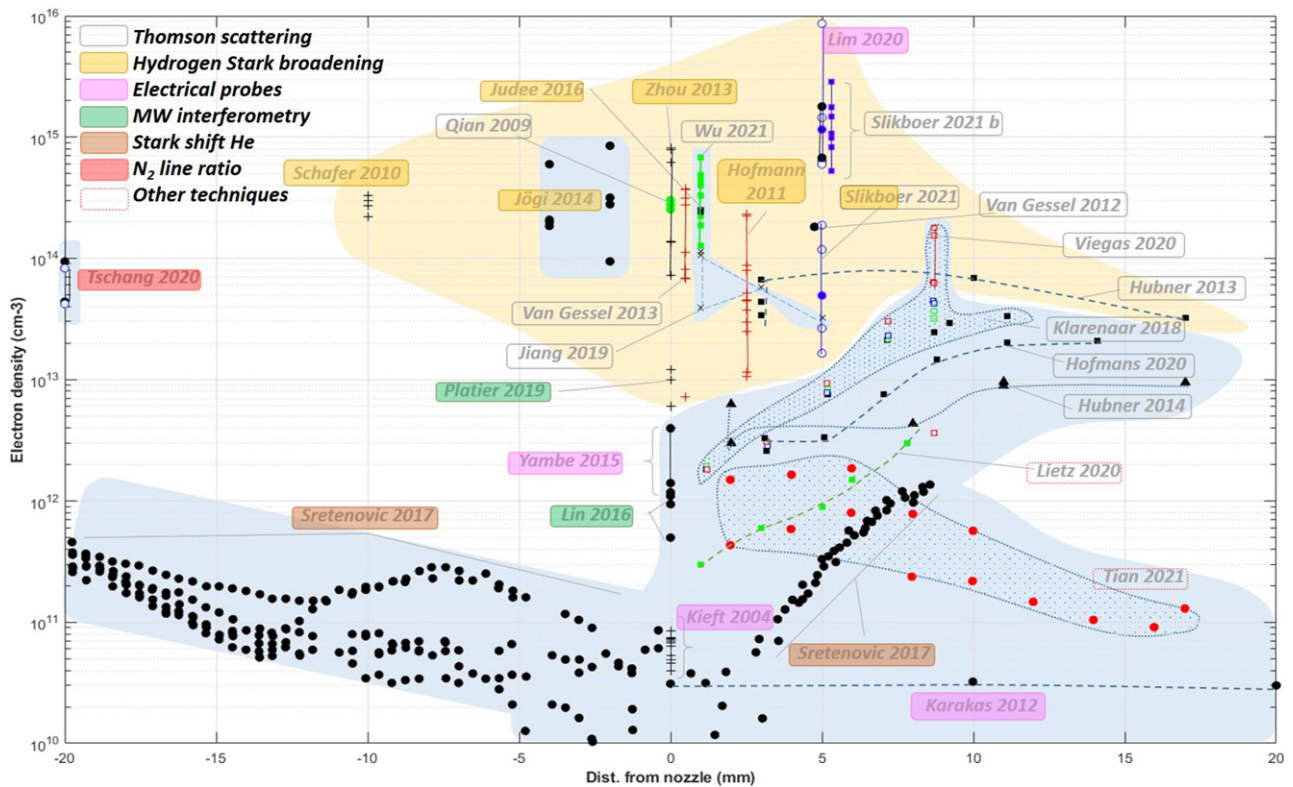
Figure 2. Experimental values from literature of electron density as function of distance from the nozzle located at x = 0 . Power sources: kHz sinusoidal ● rectangular pulses ■, short ns-pulses ▲, + RF. The symbol colours are related to the type of targets: green for dielectric targets, red for metal targets, blue for liquid targets, magenta for conductive liquid meaning saline water. Open symbols ○ are for grounded targets and solid symbols ● designate floating potential targets. The shaded blue area corresponds to jet running in helium while shaded yellow area are in argon. Coloured boxes around first author’s names designate the measurement method used. Straight lines connect minima and maxima values in series of data. Data are taken from [44, 48, 89–91, 94–101, 104, 105, 107–115].
