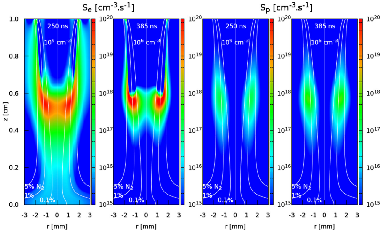
Figure 7. Cross sectional views of the ionization source terms S_e and S_p , during propagation in the plume, with L = 1.5 cm and d = 1.0 cm, 2 slm flow of He into N_2 atmosphere and V_P = +4 kV. Figure from . Reproduced with permission from [145].
