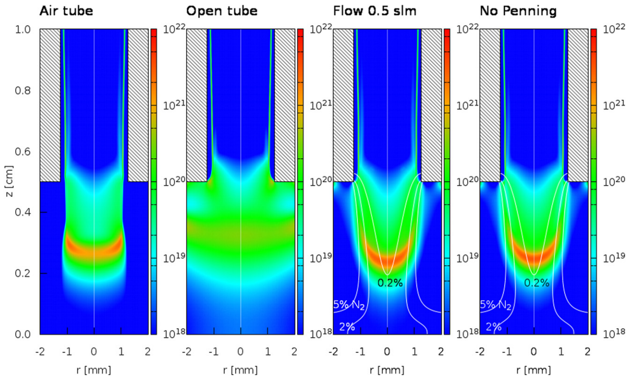
Figure 6. Cross sectional views of the total ionization source term, for several mixing conditions, at t = 170 ns, with L = 3 cm, d = 5 mm, 0.5 slm of He flowing into N_2 atmosphere and V_p = +6 kV. The white curves represent the percentage of N_2 in the He– N_2 mixture. Reproduced with permission from [145].
