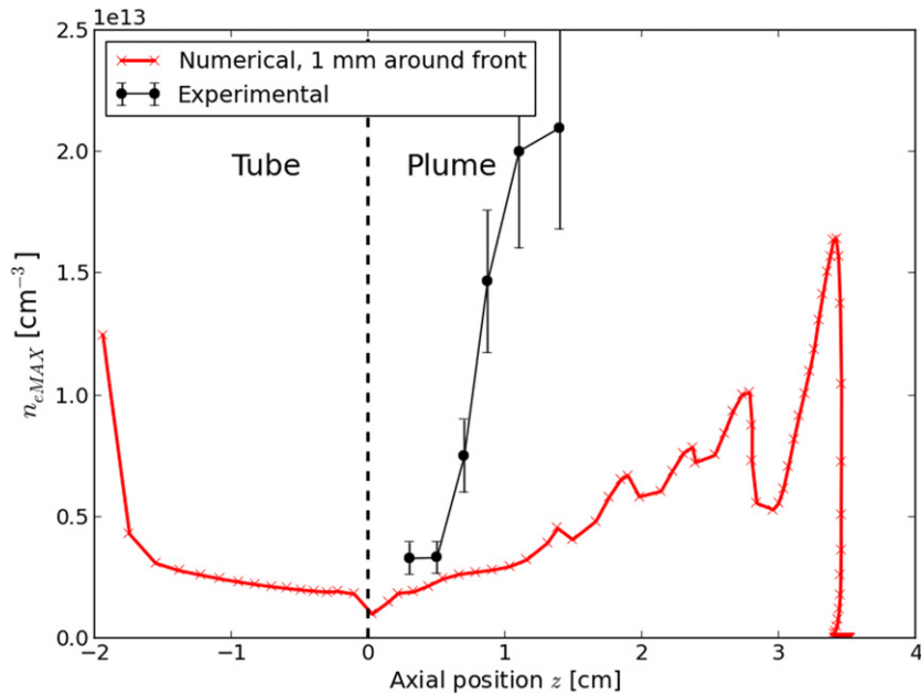
Figure 23. Electron density behind the discharge front during propagation in the tube and the plume, in experiments and simulations. Reproduced from [96]. © IOP Publishing Ltd. All rights reserved.
