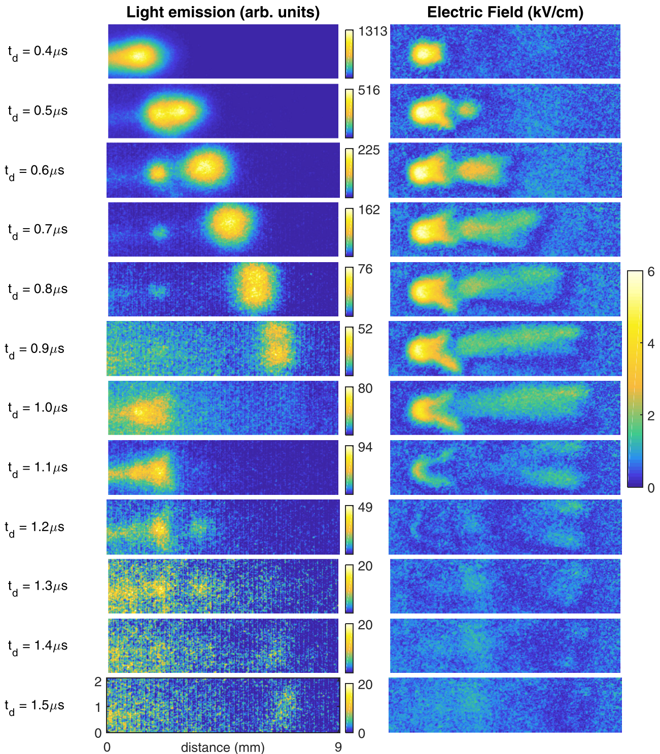
Figure 20. Plasma–target interaction for a pulsed helium jet ( V_p = +4 kV, t_f = 1 \mu\text{s} , f = 5 kHz) impacting a dielectric BSO target at 45 degrees inclination from the left-hand side at a distance of 1.2 mm, showing both the light emission from the discharge and the resulting induced electric field inside the target as a result of deposited surface charges. Time resolved measurements of 100 ns were performed. Reproduced with permission from [70].
