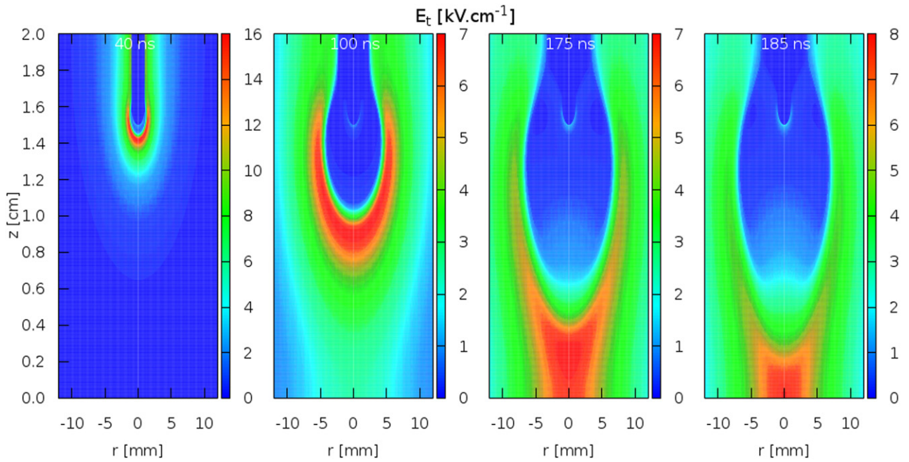
Figure 8. Cross sectional views of the magnitude of the electric field at t = 40, 100, 175 and 185 ns, in a point-to-plane discharge without tube, for V_P = +4 kV. Reproduced with permission from [145].
