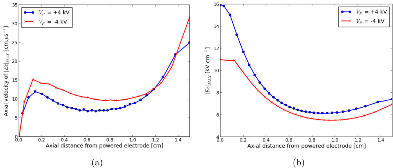
Figure 9. (a) Axial velocity of propagation and (b) magnitude of |E_z|_{\text{MAX}} between the powered electrode and the target, with 5 ns temporal resolution, for a 2 cm long domain without tube and with a grounded target, for both polarities. Reproduced with permission from [145].
