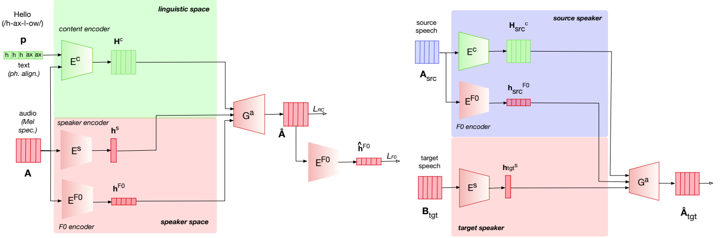
Fig. 1. Architecture of the proposed S2S-VC system. On left: The original VC comprises linguistic and speaker encoder E^c and E^s , and a decoder G^a which reconstructs the speech signal \hat{A} conditioned on content embedding H^c and speaker embedding h^s . A F0 encoder E^{F_0} is added to encode the sequence of F0 values from the original Mel-spectrogram, and a F0 loss is computed between the F0 of the reconstructed speech signal and the one of the original speech signal. On right: During conversion, content embedding H_{src}^c and F0 h_{src}^{F_0} is extracted from speech signal of the source speaker and the speaker embedding h_{tgt}^s of the target speaker.
