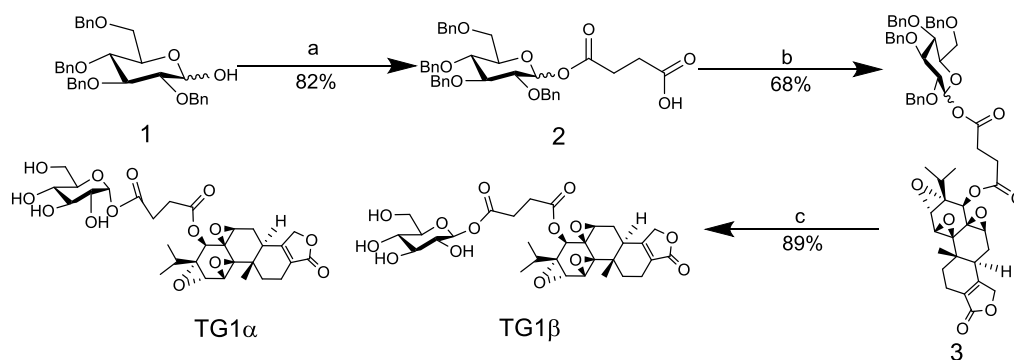
Scheme 1. Synthesis of compounds TG1. Reagents and conditions: (a) succinate anhydride, DCM, DIPEA, 82%; (b) triptolide, EDCI, DMAP, DCM, RT, 20 h, 68%; (c) H 2 , Pd/C, MeOH, THF, RT, 3 h, 89%.
