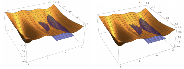
Fig. 6: Pairing by persistence on a Morse function: we compute the plane whose height is reaching f(\mathbf{x}_{\text{sad}}) (see the left side), which allows us to compute C^{\text{sad}} , to deduce the components C_i^f whose closure contains \mathbf{x}_{\text{sad}} , and to decide which representative is paired with \mathbf{x}_{\text{sad}} by persistence by choosing the one whose height is the greatest. We can also observe (see the right side) the merge phase where the two components merge and where the component whose representative is paired with \mathbf{x}_{\text{sad}} dies.
