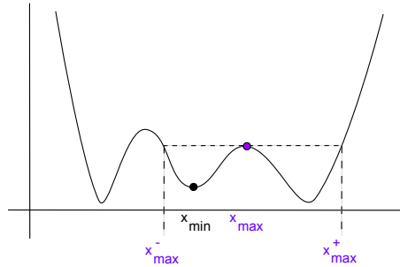
Fig. 7: Pairing by dynamics implies pairing by persistence in 1D: when \mathbf{x}_{\text{min}} (in black) is paired with \mathbf{x}_{\text{max}} (in purple) by dynamics, we observe easily that \mathbf{x}_{\text{min}} is the representative of the basin where it lies. Furthermore, the optimal path descending lower than f(\mathbf{x}_{\text{min}}) goes on the right side and goes through \mathbf{x}_{\text{max}} (since we look for a minimal effort and f(\mathbf{x}_{\text{max}}^2) is greater than f(\mathbf{x}_{\text{max}}) ). This implies that the right basin contains a representative lower than f(\mathbf{x}_{\text{min}}) . Since \mathcal{CC}([f \leq f(\mathbf{x}_{\text{max}})]) , \mathbf{x}_{\text{max}} is made of the two described basins, we obtain easily that \mathbf{x}_{\text{max}} is paired with \mathbf{x}_{\text{min}} by persistence.
