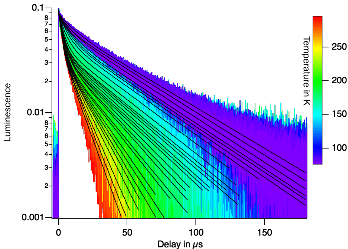
Figure 4. The fluorescence decays of [\text{Cu}(\text{IPr})(\text{dpa})][\text{PF}_6] crystals as a function of temperature. The decays were fitted as bi-exponentials. The long-lived decay is from the unquenched population. The fluorescence lifetime decreases with temperature because of the thermal activation of triplets into singlets. The fast decay at short time comes from the quenched population. From the amplitude of the fluorescence drop due to this fast component, we can measure the number of quenchers in the quenching volume around the excited states using equation (1).
