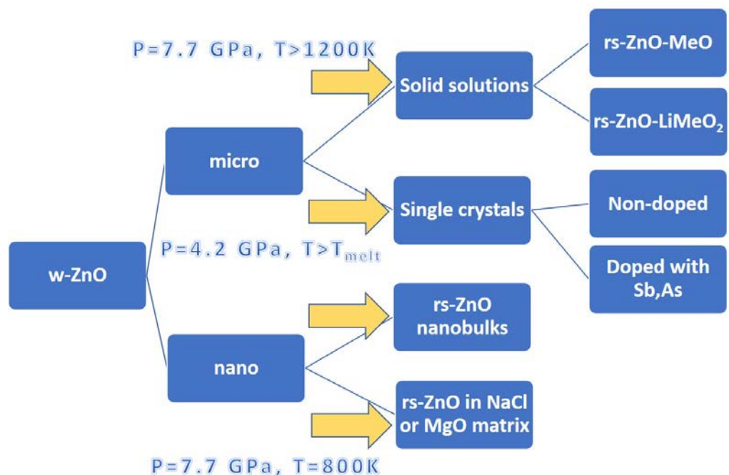
Figure 1. The scheme of high-pressure production of new phases, morphological forms and solid solutions based on zinc oxide.
