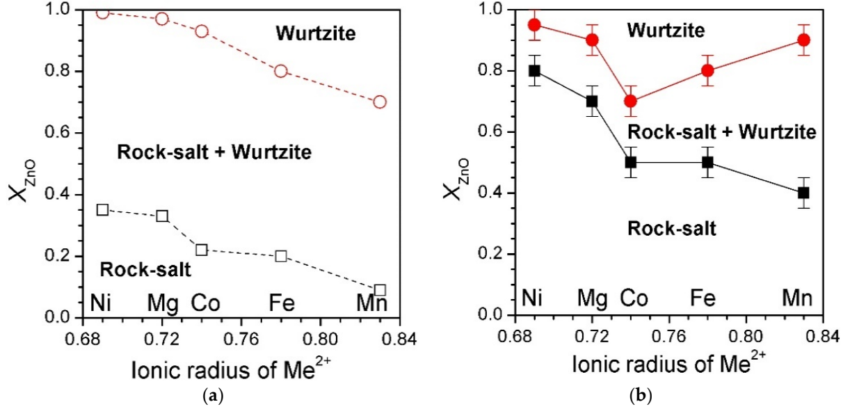
Figure 4. Phase composition in the ZnO-MeO systems as a function of the Me 2+ ionic radius: (a) at ambient pressure and 1100 K [7,46]; and (b) after quenching from 7.7 GPa and 1500 K [15,39,40].
