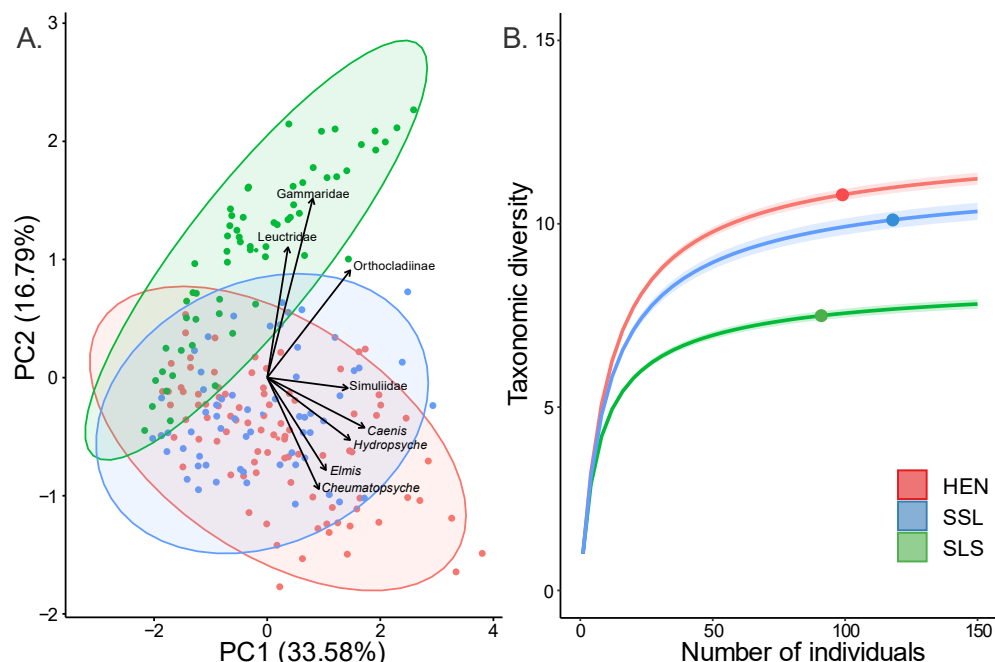
Figure 2. The macroinvertebrate community. (A) Principal component analysis (PCA) biplot performed on macroinvertebrate abundances (log 10 (x + 1) transformed). (B) Taxonomic diversity ( 1 D) and 95% CIs (shaded area) of the macroinvertebrate community. Dots indicate the estimate of taxonomic diversity standardised at 95% sample coverage.
