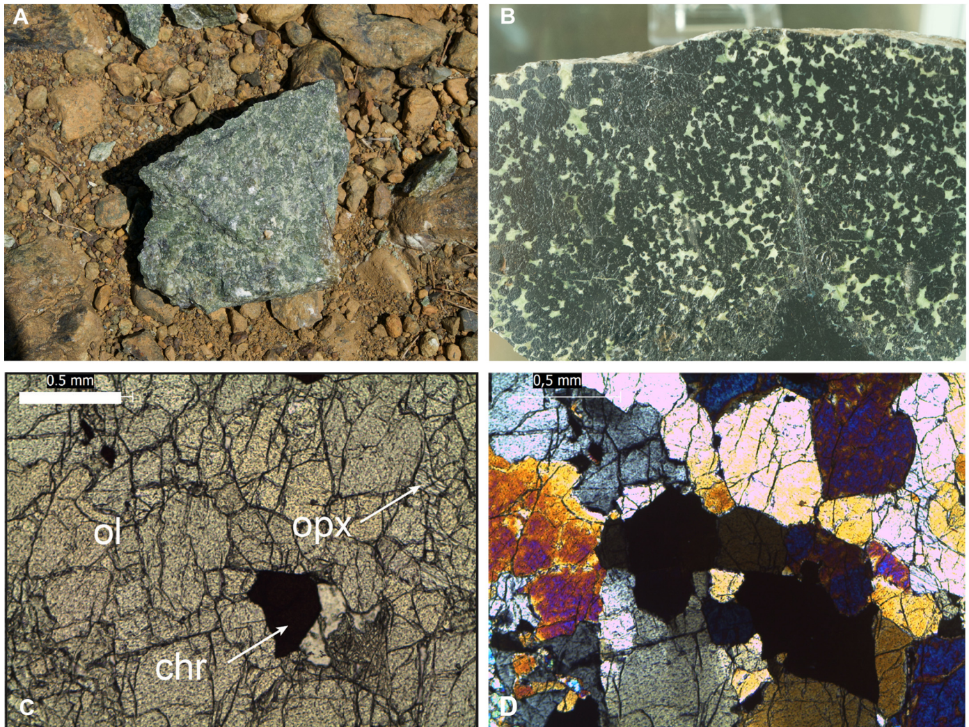
Fig. 2. A: Fragment of unserpentinized harzburgite from Me Maoya freshly broken from massive (<math><2\text{ m}^3</math>) boulder littering the bed of Baraoua River draining the southern flanks of Me Maoya massif NE of Bourail. B: Example of the podiform chromitite ore from collections of the Tiébaghi Historical Society in the museum at the former Tiébaghi mine village. C: Photomicrograph of unserpentinized harzburgite from the Me Maoya Massif collected from the Baraoua River (plain polarised light) ol = olivine, opx = orthopyroxene, chr = chromite). D: Photomicrograph of unserpentinized harzburgite from the Me Maoya Massif collected from the Baraoua River (cross-polarised light).
