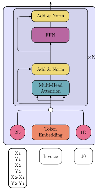
Fig. 1: LayoutLM architecture. Token embeddings are enriched with 1D positional encoding and 2D spatial encoding specific to this architecture. The number of blocks N varies from 12, for the base model, to 24, for the large one.
