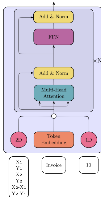
Fig. 1: LayoutLM architecture.
