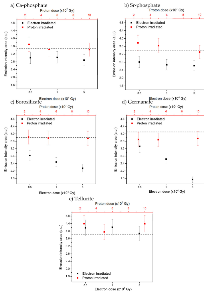
Figure 5. \text{Yb}^{3+} emission intensity area ( \lambda_{\text{exc}} = 963 nm) after irradiation with varying doses for Ca-phosphate (a), Sr-phosphate (b), borosilicate (c), germanate (d) and tellurite (e) glasses, respectively. Dashed line shows emission intensity area for as-prepared samples, error bars \pm 10\% .
