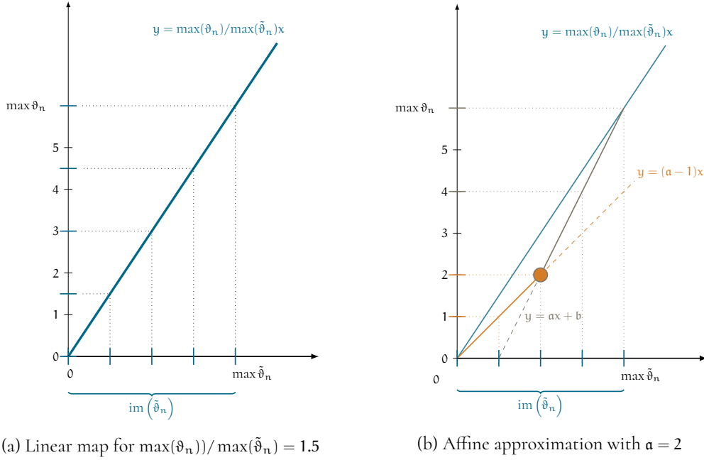
Figure 14: Affine approximation
