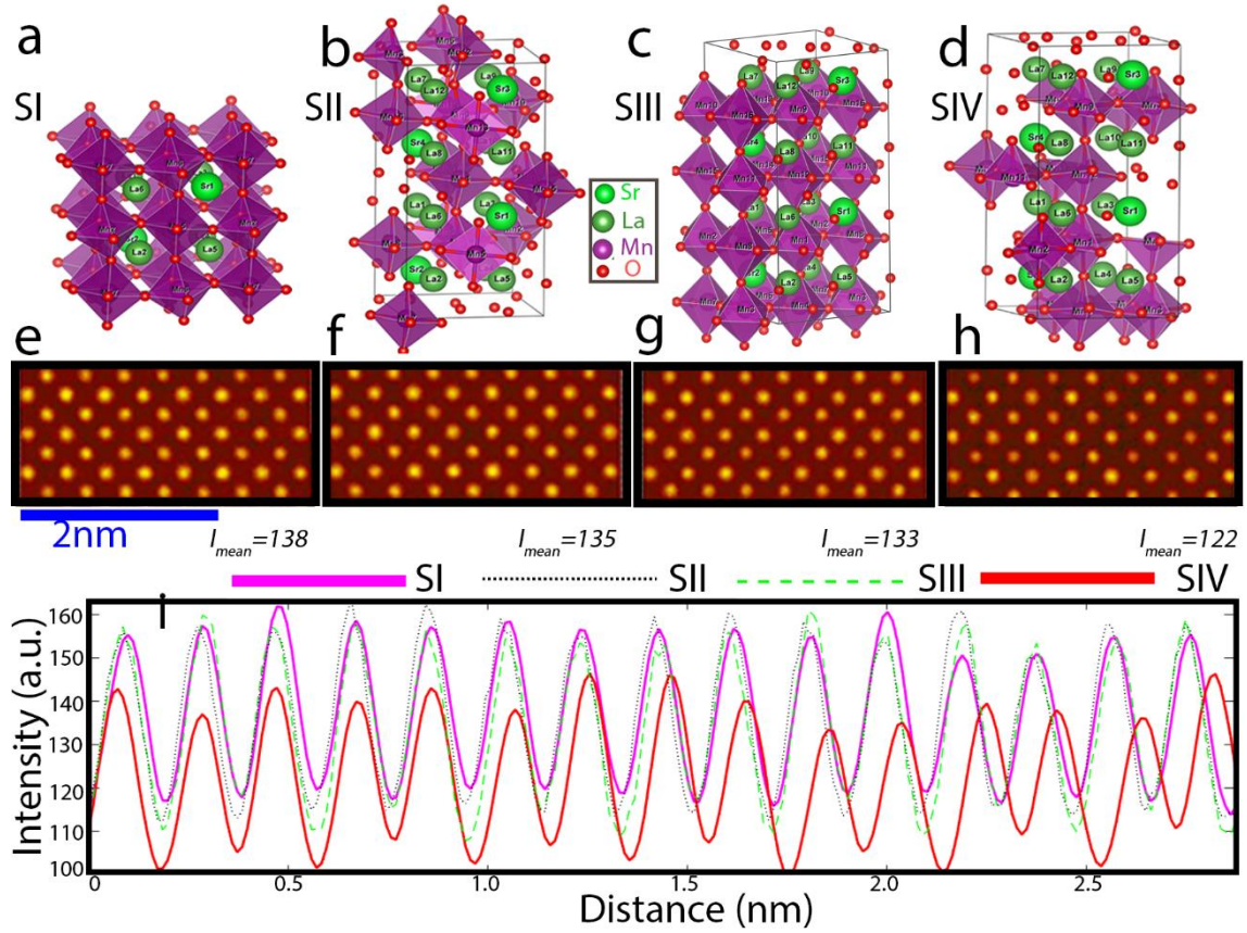
Figure 5: Atomistic simulation results. (a-d) Represent the 3D view of the energetically relaxed structures by DFT calculation for structure SI, SII, SIII, and SIV, respectively. The incomplete polyhedral shows the position of oxygen vacancies at the other end of the polyhedral (e-h) multislice simulated STEM-ADF images of the [010] orientated LSMO structure with 15 nm thickness using the corresponding structures. The scale bar is the same for all the simulated images. (i) Intensity profile calculated from each simulated STEM-ADF image.
