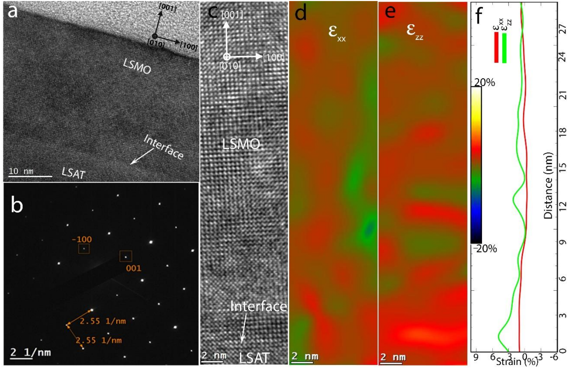
Figure 1: Cross-sectional HRTEM image and corresponding strain analysis: (a) HRTEM image of [001] oriented LSMO thin film grown on LSAT substrate, (b) SAED pattern from the imaged region (c) Experimental HRTEM image used for strain analysis (d,e) symmetric strain components: in-plane ( \epsilon_{xx} ), out-of-plane ( \epsilon_{zz} ), respectively. A color bar for the strain map is shown. (f) Line profiles of the strain components, averaged over the width of the strain maps in the [100] direction of the film. All strain values indicated in this figure are in percentage.
