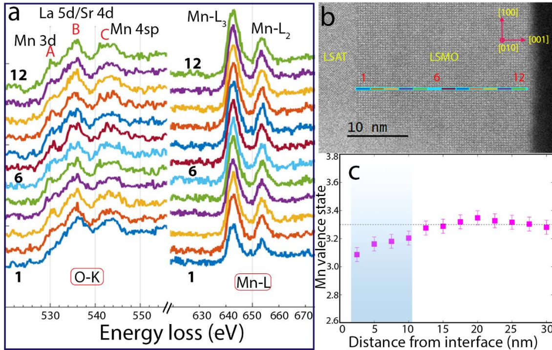
Figure 3: EELS analysis of the Mn oxidation state in the film region. (a) Fine structures of O-K and Mn-L edges. Three prominent peaks for O-K edges are labeled as “A”, “B”, and “C”. Peaks “A” and “C” correspond to O 2p – Mn 3d and 4sp hybrid states, respectively, while peak “B” is characteristic of O 2p Sr 4d or La 5d hybrid states. The energy difference \Delta E between peaks “A” and “B” was measured to determine the Mn valency. (b) STEM-HAADF image of the LSMO/LSAT structure and the line shows the area from where EELS line profiles have been collected. The numbers indicate the area across which the average spectra were collected. (c) Estimated Mn valence in the LSMO film as a function of distance from the interface with the substrate.
