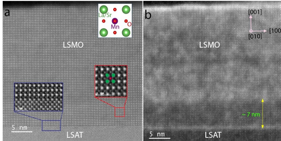
Figure 2: Experimental high-resolution STEM images. (a) STEM-HAADF image showing the cross-sectional geometry of the LSMO/LSAT heterostructure along the [010] zone axis. The inset in the blue box shows that the interface is atomically flat and defect free. The inset in the red box shows a close-up image of the LSMO thin film. The scale bar of the insets corresponds
