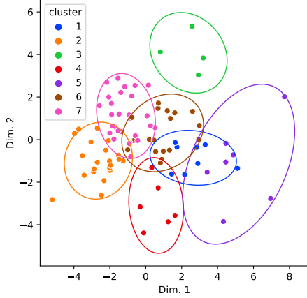
Figure 2: Visual representation of the KMeans clusters on the plane directed by the two dimensions of the PCA. The ellipses have been drawn using radiuses equals to 2\sigma .
