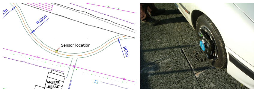
Figure 2. left: Sensor location in the curved test track; right: sensor under the vehicle instrumented wheel
