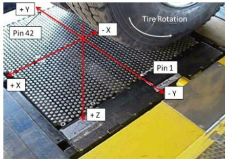
Figure 1. Stress-In-Motion (SIM) system (source: [9], fair use)
