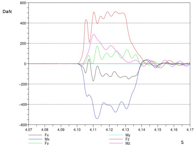
Figure 4. Road sensor measurements (DaN and N.m) in function of time (s); B70 speed case
