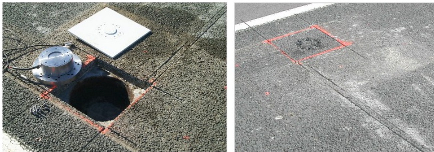
Figure 1. Road sensor: sensor detailed view (left), and final installation in the road pavement (right)
