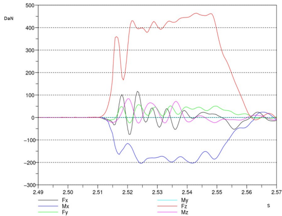
Figure 3. Road sensor measurements (DaN and N.m) in function of time (s); V40 speed case
