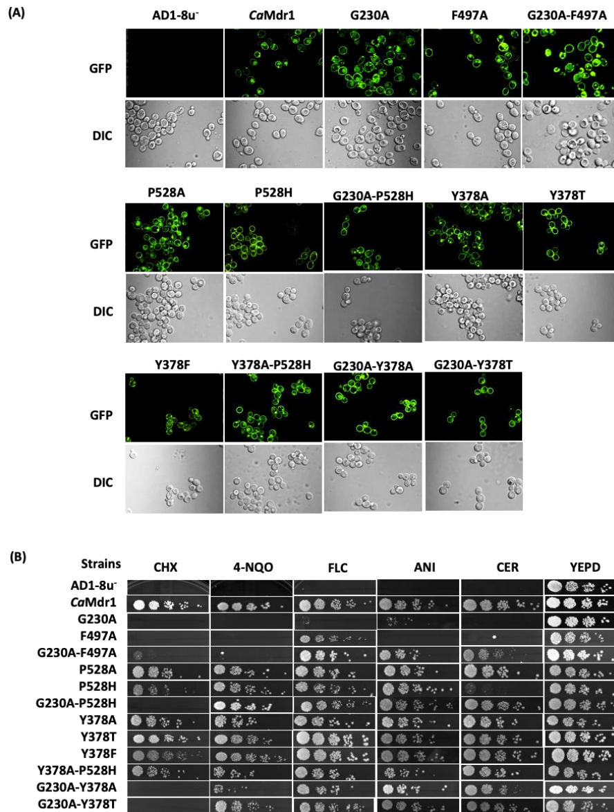
Figure S8. Phenotypic characterization of yeast strains expressing single secondary mutants of CaMdr1 . (A) Fluorescence imaging by confocal microscope showing PM localization of AD1-8u r (control), CaMdr1 -GFP (WT), mutant and reconstructed suppressor with corresponding differential interference contrast (DIC) images and merged images. (B) Comparison of growth by spot dilution assays for mutant variants on different CaMdr1 substrates as CHX (0.1 mg/L), 4-NQO (0.15 mg/L), FLC (0.8 mg/L), ANI (10 mg/L) and CER (4 mg/L) in YEPD agar plates. Images were captured after 48 hours of incubation at 30 °C.
