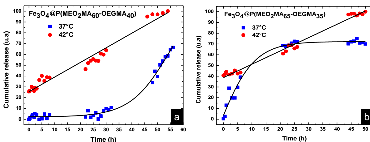
Figure 7. Release of DOX from \text{Fe}_{3-\delta}\text{O}_4@\text{P}(\text{MEO}_2\text{MA}_{60}\text{-OEGMA}_{40}) and \text{Fe}_{3-\delta}\text{O}_4@\text{P}(\text{MEO}_2\text{MA}_{65}\text{-OEGMA}_{35}) MNPs in physiological medium (DMEM).
