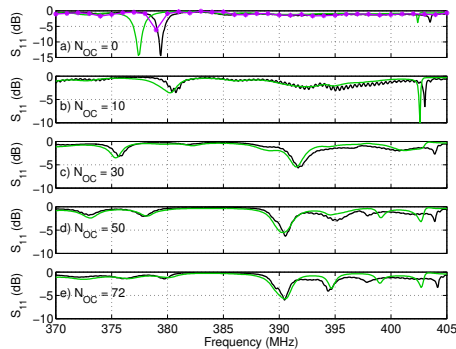
FIG. 6. Simulated (green) and measured (black) S_{11} magnitude spectra for resonators with N_{OC} = 0, 10, 30, 50, and 72 . Port Impedance is 50 \Omega . For the N_{OC} = 0 case, the complete resonator simulation is also shown (magenta).
