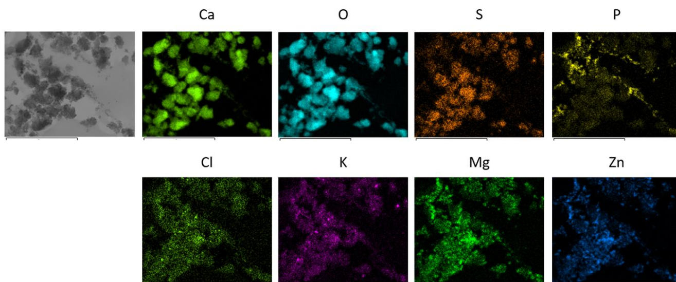
Figure 2. HR-TEM mapping of Eco-base-Ah (scale bar: 1 μm).
