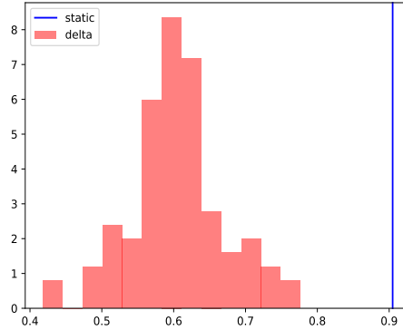
Figure 3.2: The red histogram is the density of -pnl_1 + HVA_1 - HVA_0 conditional on model switch occurring, i.e. on \{0 < \tau_s \leq 1\} , for delta hedging without frictions. The vertical blue line in the right panel corresponds to the deterministic loss -pnl_1 + HVA_1 - HVA_0 = K + HVA_1 - HVA_0 for static hedging, also conditional on \{0 < \tau_s \leq 1\} . Note that, in both cases, HVA_1 - HVA_0 = 0 - K(1 - e^{-\lambda T}) \simeq 0.095 on \{0 < \tau_s \leq 1\} .
