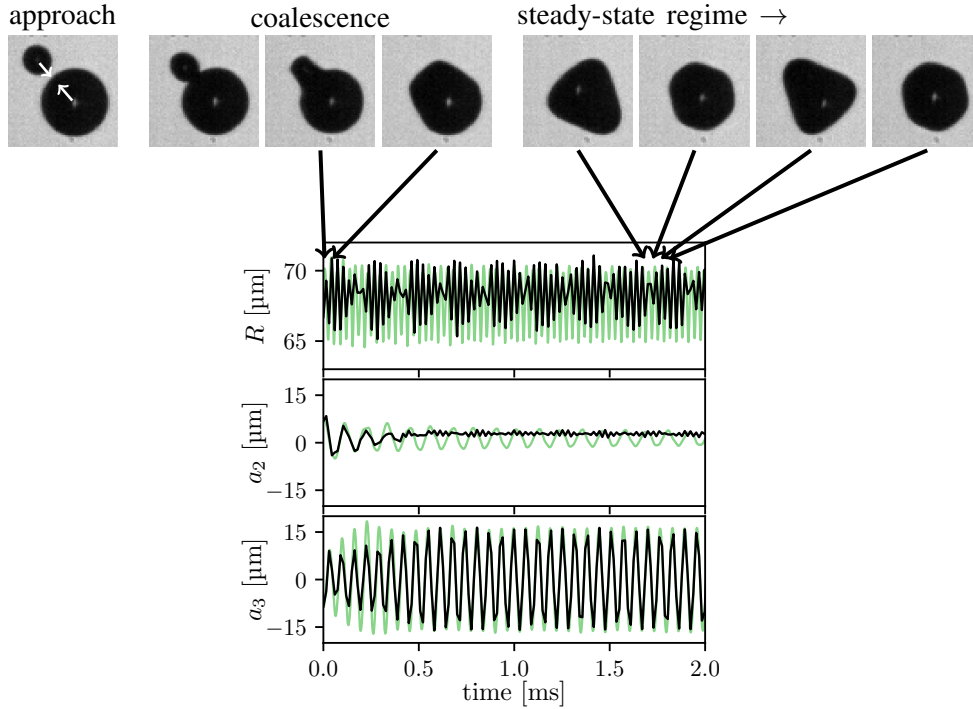
Figure 2. Example snapshot of bubble coalescence (frame size 220 \times 220 \mu\text{m} ). After the approach, the two bubbles coalesce at the time defined as t = 0 \text{ ms} . After a relatively short time, the steady-state regime is reached. The plot shows the modal decomposition for the radial mode R and the modes 2 and 3. As can be seen on the snapshots, the modals amplitude a_2 becomes negligible while the maximum modal amplitude a_3 reaches a steady state value. Note that the experimental values (black line) are superposed with a numerical simulation (green line) according to the coupled-mode theory of volumic and nonspherical oscillation [8].
