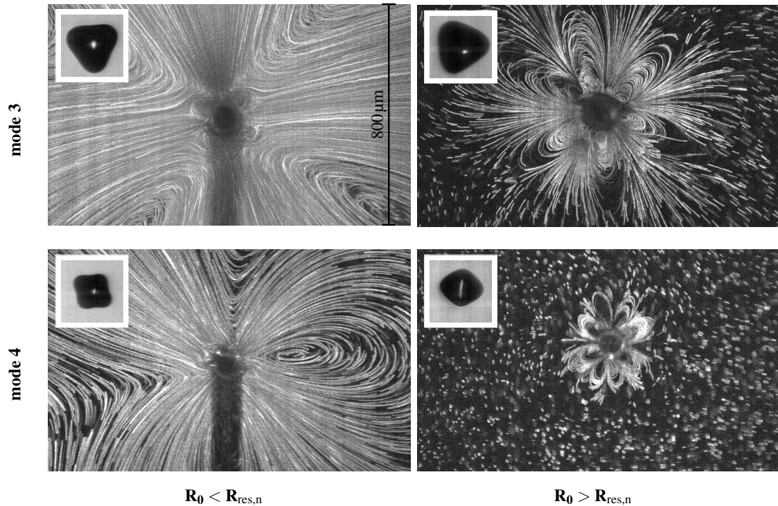
Figure 4. Four examples of microstreaming patterns. The upper row shows two examples for a mode 3, the lower row two examples for a mode 4 (see snapshots of the respective dynamics in the respective inlets). Two types of patterns are observed: the examples on the left are large cross-like patterns for bubbles that are smaller than the respective resonant size ( R_{\text{res},3} \approx 54\mu\text{m} and R_{\text{res},4} \approx 67\mu\text{m} ), the examples on the right are confined lobes patterns for bubbles that are larger than the respective resonant size. The radii are in the upper left case R_0 \approx 65\mu\text{m} , in the upper right R_0 \approx 70\mu\text{m} , in the lower left R_0 \approx 53\mu\text{m} , and in the lower right R_0 \approx 55\mu\text{m} .
