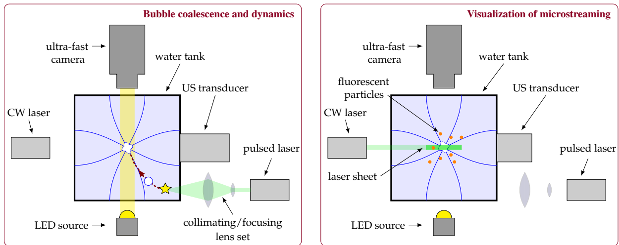
Figure 1. Schematic representation of the experimental setup; left : creation of bubbles by short laser pulses, trapping in the acoustic field and triggering of surface modes via bubble coalescence. The camera and light source allow the visualization of the bubble dynamics; right : visualization of microstreaming with fluorescent tracer particles and a laser sheet.
