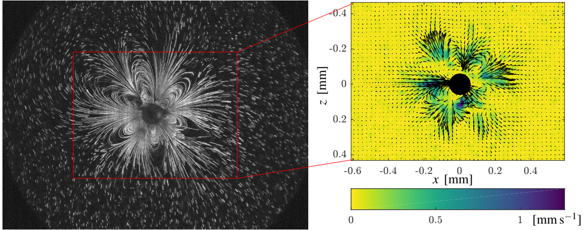
Figure 3. Microstreaming around a bubble oscillating on a mode 3. On the streak image (left), six lobes are visible. The PIV result reveals maximum velocities of the order of 1 \text{ mm s}^{-1} .
