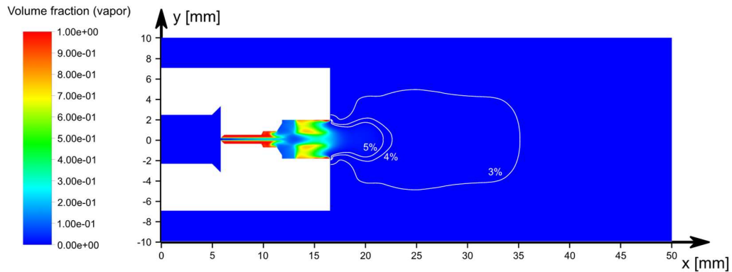
Figure 3. Distribution of volume fraction of vapor at 5.65 ms. The white contour lines from outside to inside represent the contours with volume fraction of vapor 3%, 4% and 5% respectively.
