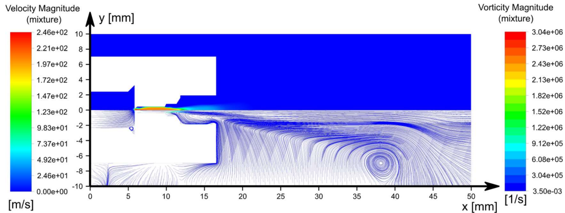
Figure 2. The upper half of the image is the velocity distribution represented by the contour map and the vorticity magnitude is represented by the path-line diagram in the lower part at 5.65 ms.
