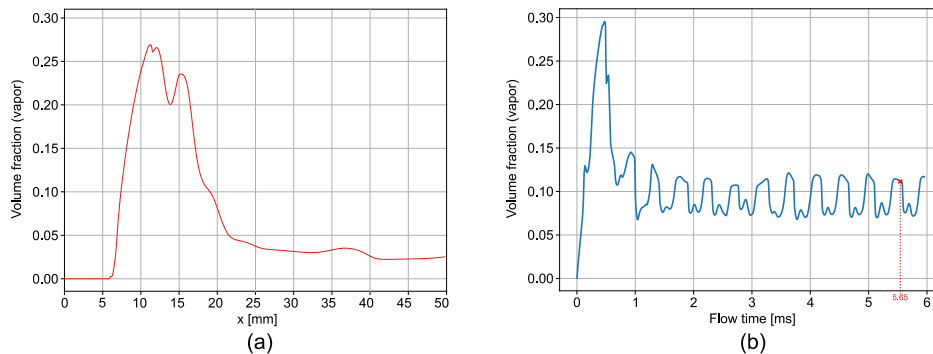
Figure 4. (a) Distribution curve of volume fraction of vapor on the axis of symmetry at 5.65 ms; (b) The curve of the average value of vapor volume fraction on the characteristic surface over time. The average fluctuation period is 0.43 ms.
