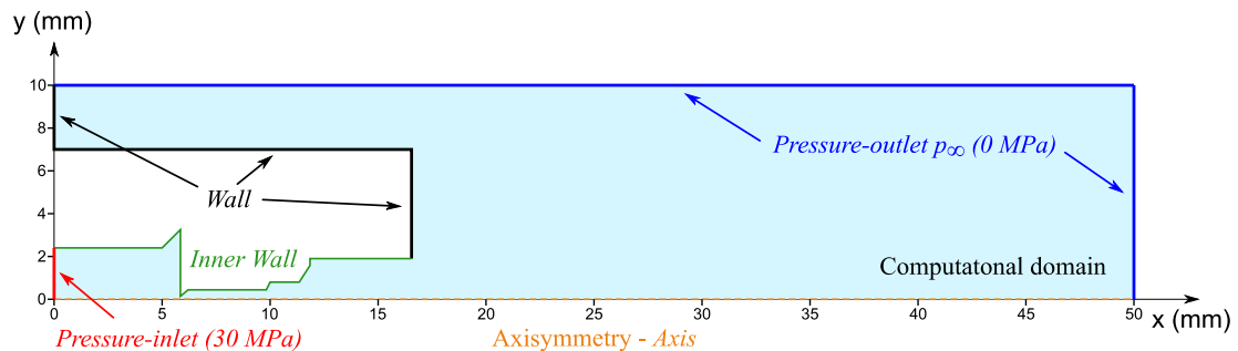
Figure 1. Schematic representation of the model geometry used to simulate cavitation jet. The inner wall (green border) hypothesis satisfies the no-slip boundary condition and the outer wall (black border) satisfies the slip boundary condition.
