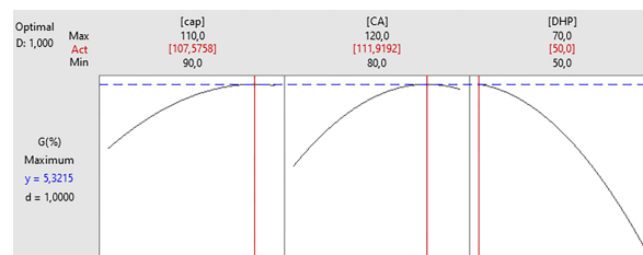
Fig. 6. Response optimisation of the grafting process. CA, citric acid; DHP, disodium hydrogen phosphate
