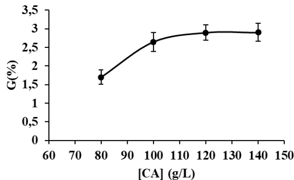
Fig. 3. Effect of the CA crosslinking agent concentration on the fabric mass gain. CA, citric acid
