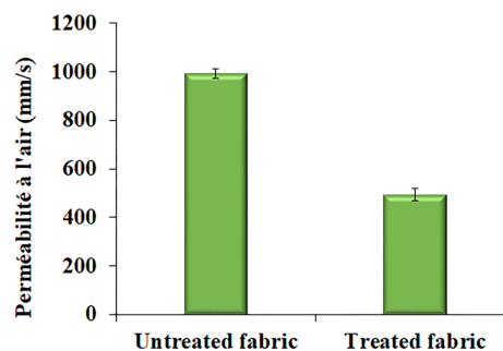
Fig. 10. Air permeability of knitted cotton fabrics before and after grafting
