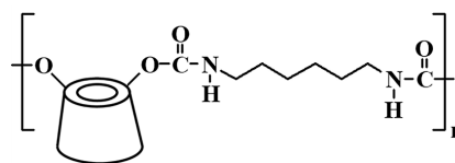
Fig. 1. Molecular structure of the PU polymer based on \beta -cyclodextrin forming the microcapsules shell. PU, Polyurethane
