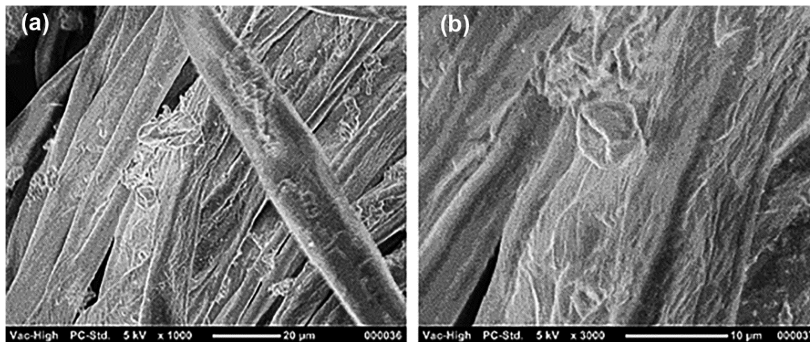
Fig. 11. SEM micrographs of knitting grafted with fragrant microcapsules after 40 washing cycles at (A) \times 1,000 and (B) \times 3,000 magnification. SEM, scanning electron microscopy
