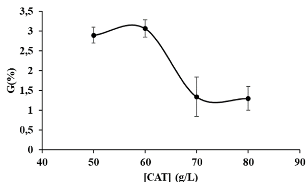
Fig. 4. Effect of the DHP CAT on the mass gain. CAT, catalyst concentration; DHP, disodium hydrogen phosphate
