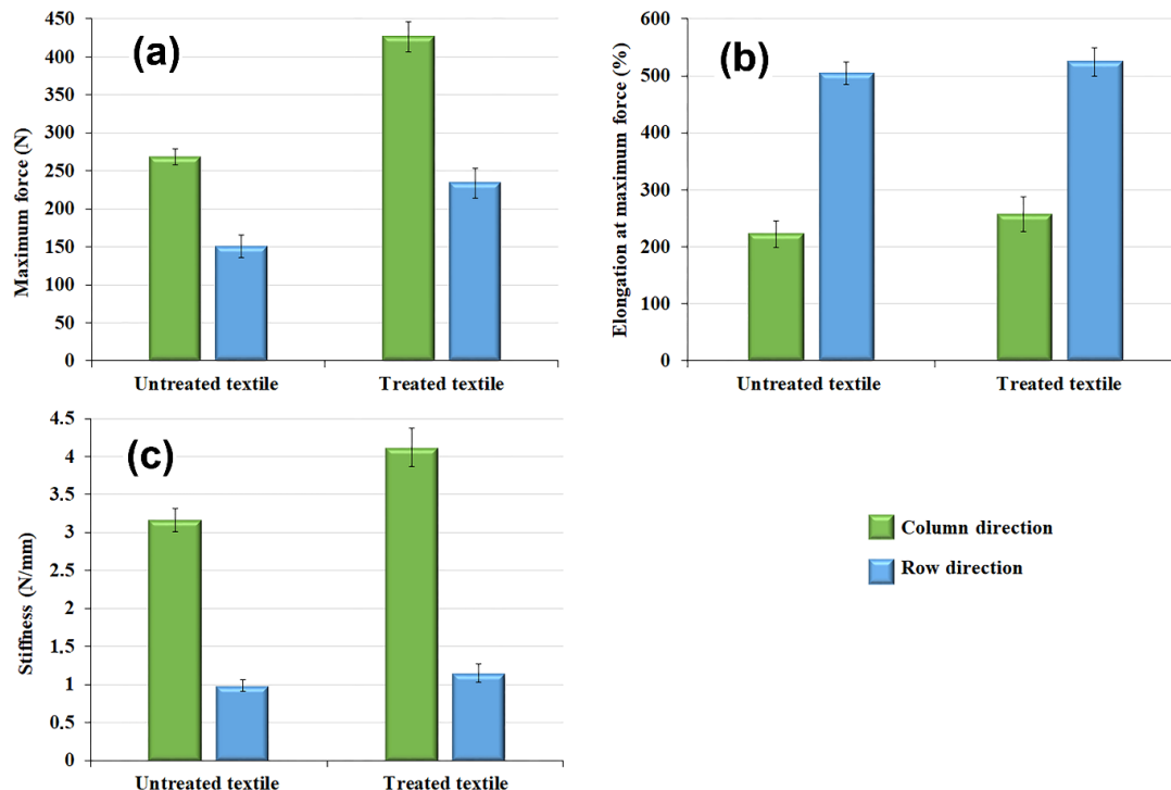
Fig. 9. Variation of: (A) maximum force, (B) elongation at maximum force and (C) stiffness before and after grafting treatment in row and column directions
