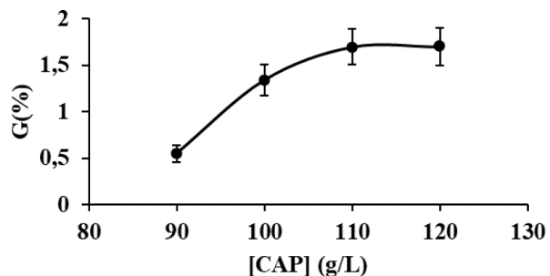
Fig. 2. Effect of the microcapsules concentration (CAP) on the mass gain G
