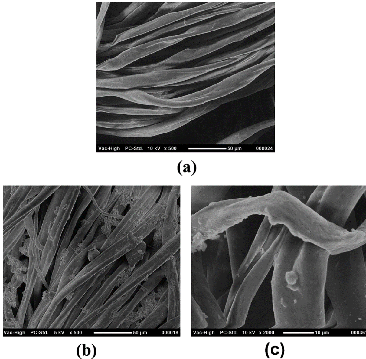
Fig. 7. SEM micrographs of: (A) untreated cotton knitted textile at \times 500 magnification and (B, C) treated cotton knitted textile at \times 500 (B) and \times 2,000 (C) magnifications. SEM, scanning electron microscopy
