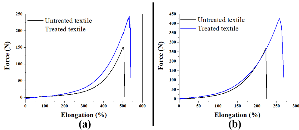
Fig. 8. Tensile behaviour of untreated and treated knitted fabric in both directions: (A) row direction and (B) column direction
