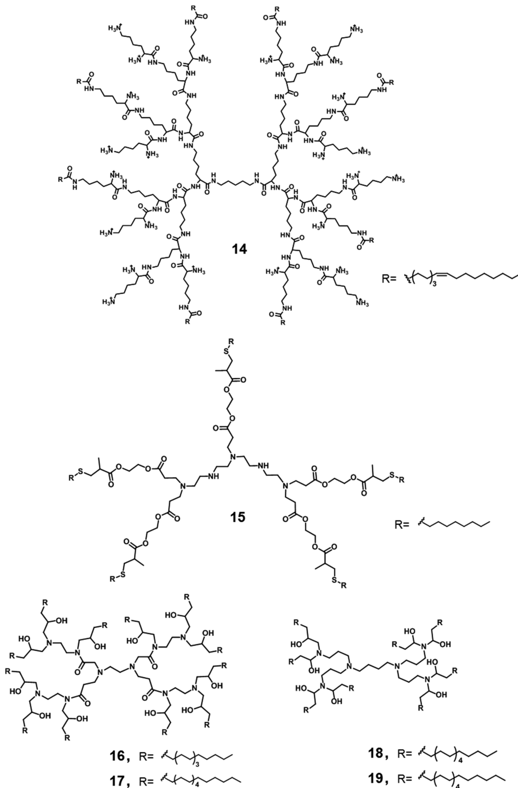
Figure 8. Examples of core-shell type amphiphilic dendrimers established for siRNA delivery. 13,15,43,45 Adapted with permission from ref 13 (Copyright 2014 Wiley-VCH Verlag GmbH & Co. KGaA), ref 15 (Copyright 2016 National Academy of Sciences), ref 43 (Copyright 2007 American Chemical Society), and ref 45 (Copyright 2015 American Chemical Society).
