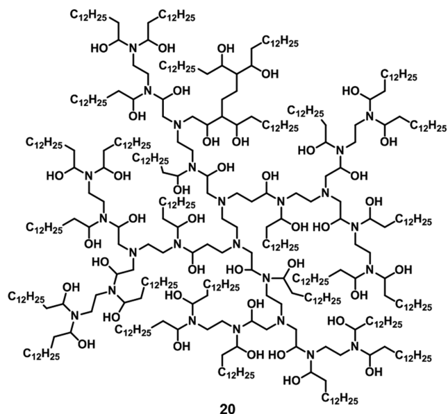
Figure 9. Amphiphilic dendrimer 20 developed for the delivery of mRNA vaccines. 48 Adapted with permission from ref 48 (2016 National Academy of Sciences).
