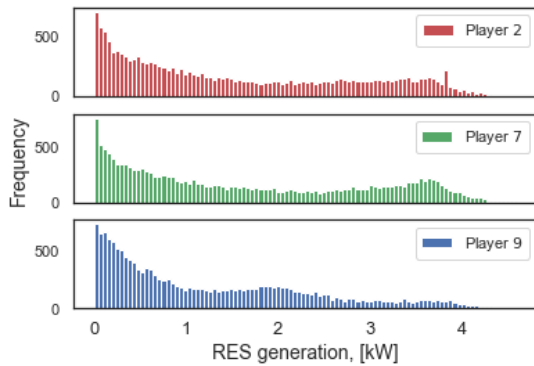
Figure 4 Histograms of RES-generation.
