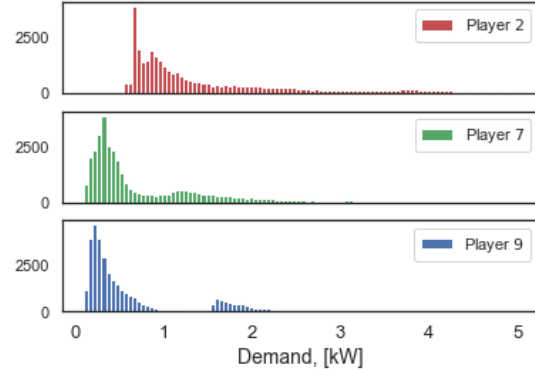
Figure 5 Histograms of demand.
