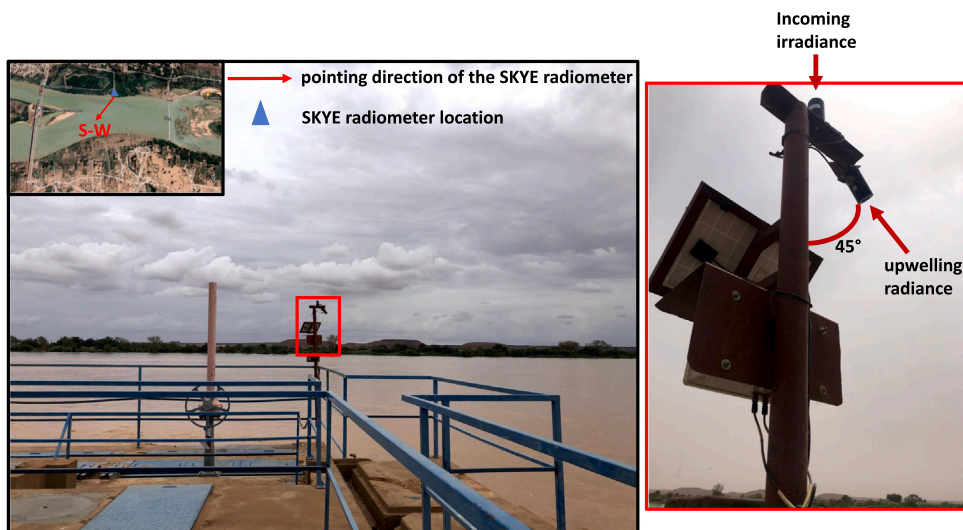
Fig. 3. SKYE radiometer at the Sampling station monitoring Niger River water reflectance.
