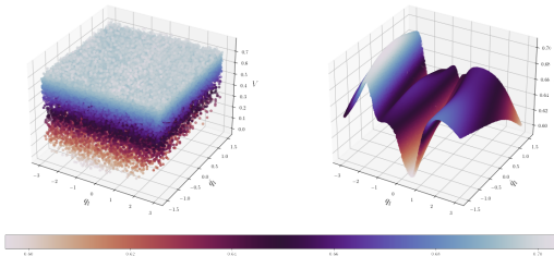
Fig. 5: The Figure on the left shows the predictions for value functions of V_\alpha^{n=10} for the 14 dimensional state space of the manipulator arm. The points were randomly sampled from 14 dimensional space. In the Figure on the right, only q_1, \dot{q}_1 were randomly sampled and the other 12 dimensions were set to 0.
