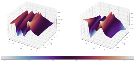
Fig. 6: Slices of the gradients of the neural network, i.e V_\alpha^{n=10} for the manipulator state space
