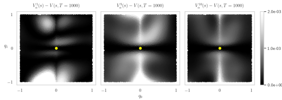
Fig. 4: Scatter plot of the distribution of mean squared errors between V_\alpha^1, V_\alpha^5, V_\alpha^{10} and V(s, T = 1000) for unicycle. The yellow dot is the goal position for the unicycle.
