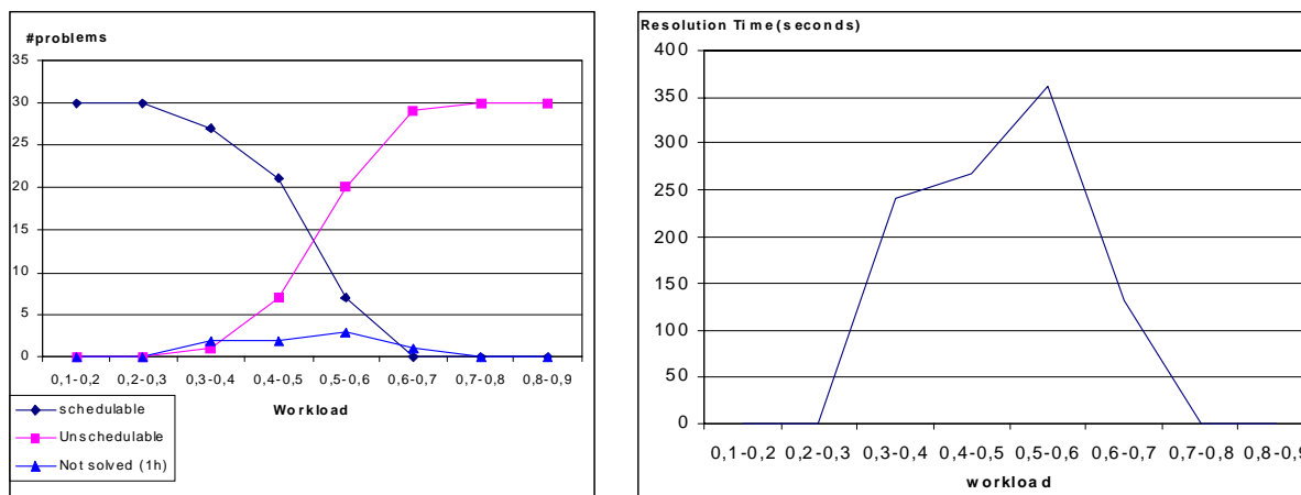
Fig. 3. Number of problems solved in 1 hour (3a) and Average resolution time in seconds (3b)
