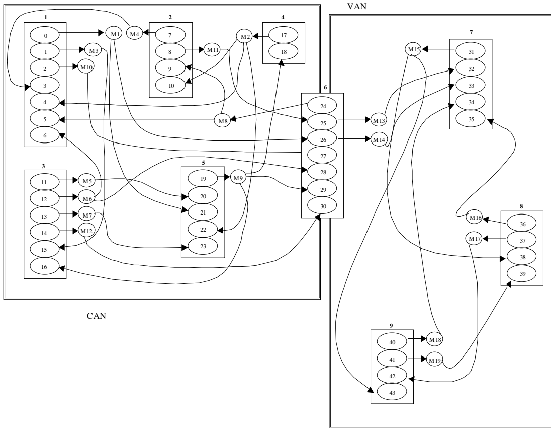
Fig. 1. Software architecture of the application
