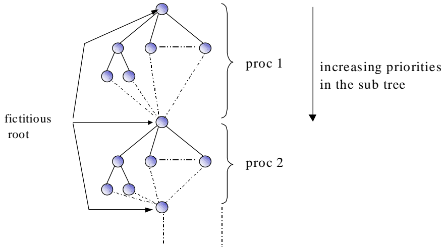
Fig. 2. Structure of the search tree
