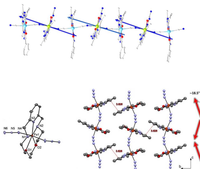
Figure 8. SCM involving PBP Fe II centres as the source of magnetic anisotropy. (top) 1D-[Fe(H 2 L1 NH2 ){Cr(L1 Ph )(CN) 2 }]·PF 6 with local easy magnetic axes depicted as blue arrows (Fe in green, Cr in light-blue). Reprinted with permission from Ref. 23 , Copyright 2022 American Chemical Society), (bottom) 1D-azido-bridged [Fe(L5 H )(N 3 )]·ClO 4 , the red arrows represents the easy axis of magnetization of a Fe II center positioned along N azido -Fe-N azido axis, thus highlighting the tilt angle at the origin of weak ferromagnetism and SCM behavior (Adapted with permission from Ref. 76 , copyright 2021 American Chemical Society).
