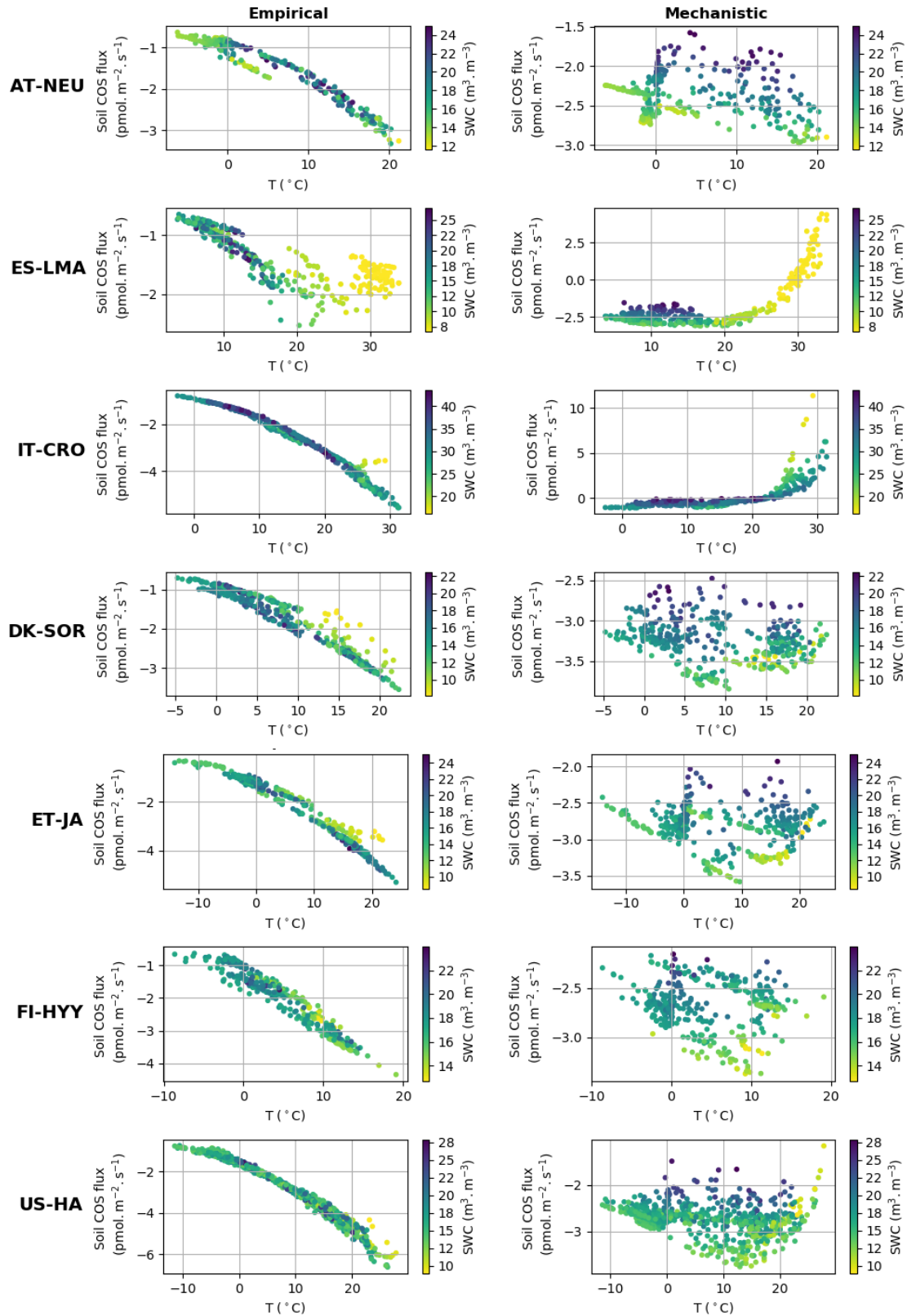
Figure 4. Simulated daily average net soil COS flux ( \text{pmol m}^2 \text{s}^{-1} ) versus soil temperature ( ^{\circ}\text{C} ) and soil water content (SWC) ( \text{m}^3 \text{m}^{-3} ) at AT-NEU, ES-LMA, IT-CRO, DK-SOR, ET-JA, US-HA, and FI-HYY, for the empirical and the mechanistic model.
