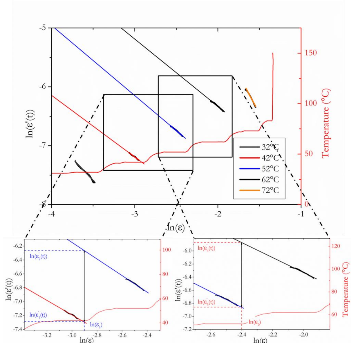
Figure 11 : The evolution of experimental (black dots) and the extrapolated (colored line) evolution of \ln(\epsilon'(t)) as a function of \ln(\epsilon) by the stepwise isothermal experiment, allowing calculation of the activation energy Q from two isotherms (Eq 11). A zoom is proposed in the range 42 and 52 ^{\circ}\text{C} and 52 and 62 ^{\circ}\text{C} for sake of clarity.
