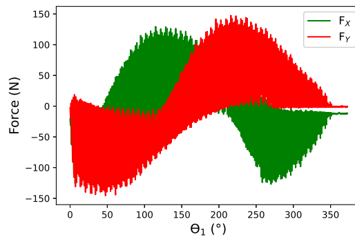
Figure 6: Experimental forces F_X and F_Y during circular milling of Aluminium as an example ( f_z=0.1 mm/th and V_c=40 m/min)
