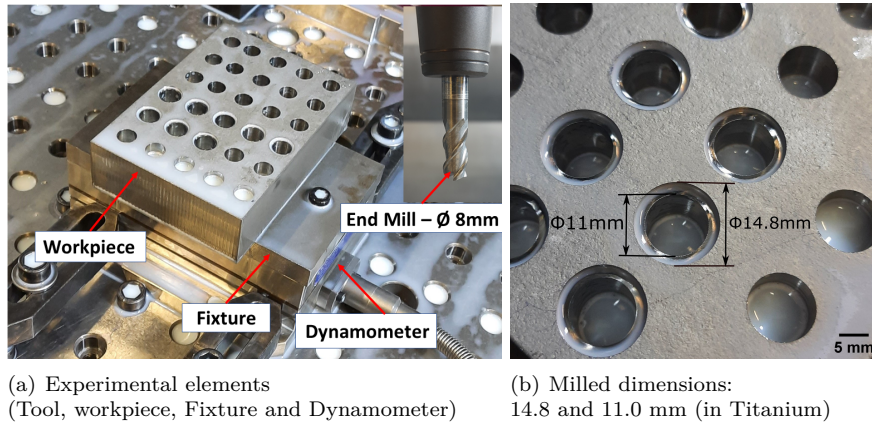
Figure 3: Experimental setup
