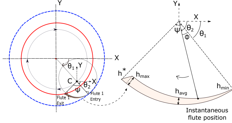
Figure 2: Chip geometry in circular milling
