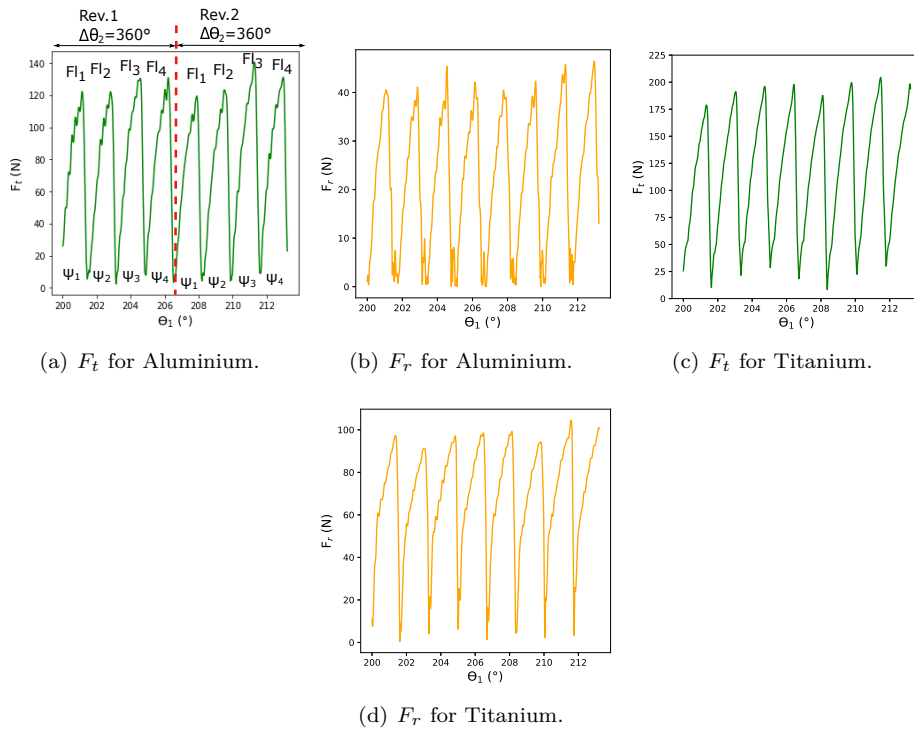
Figure 7: Calculated F_t and F_r during 2 revolutions in circular milling of Aluminium and Titanium (window on \theta_1 = [200^\circ - 213^\circ] ) at f_z = 0.1 mm/th and V_c = 40 m/min
