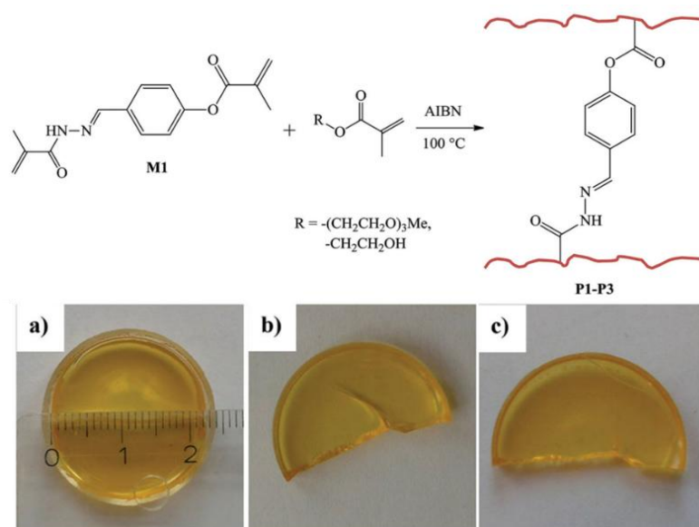
255 Figure 13 – Cross-linked film with self-healing properties. a) Polymer film, b) Film after scratch, c) Healed scratch after heating at 100°C for 64h. Adapted from Kuhl et al. 72
