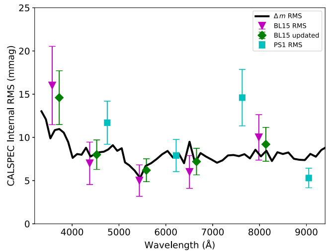
Figure 8. The dispersion of the \Delta m values ( \sigma_l from Equation (4)) for our 14 CALSPEC standards (black curve). The calculation is performed in bins of 40 wavelength samples in order to lower the uncertainty on the individual \Delta m values for stars with fewer (STIS and/or SNIFS) observations. Overplotted are the dispersions when comparing filter photometry for the UBVR filters (Bohlin & Landolt 2015; BL15 magenta diamonds). We have updated the UBVR intrinsic dispersion, including subtraction of the quoted filter photometry measurement uncertainty, to include newer space-based CALSPEC standard stars (green squares). We also plot a similar comparison that we have done for Pan-STARRS1 in the griz filters. These points have been offset slightly in wavelength for clarity. This demonstrates that the dispersion of \Delta m values determined from our Bayesian hierarchical standardization model are consistent with other external checks of CALSPEC.
