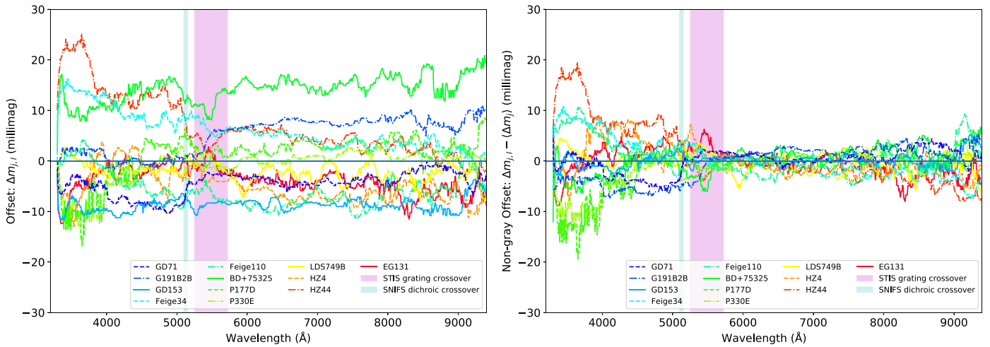
Figure 9. The \Delta m_l values for each star showing the offset with respect to CALSPEC. On the left, we show the full \Delta m_l for each star, making plain that most of the power is in the form of constant in-wavelength offsets. On the right, we have removed the constant term in order to highlight the chromatic components. The vertical blue-shaded region shows the SNIFS dichroic crossover wavelength range; there does not appear to be much structure between the blue and red sides of SNIFS. The vertical magenta-shaded band is the region where the CALSPEC HST observations change grating coverage. The values have been median-smoothed in wavelength for clarity. Only primary calibrators observed on more than one night are shown, since otherwise the per-observation repeatability dominates, forcing the \Delta m_l to fall back on the prior, \sigma_l .
