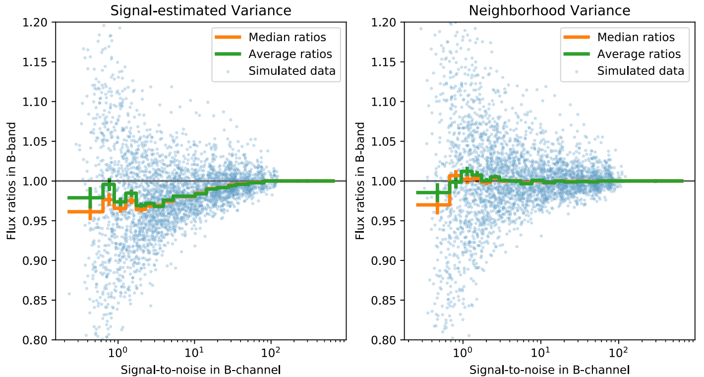
Figure 5. Results of simulations to test the linearity of our extract_star2 software that measures 1D spectra from SNIFS data cubes. On the left is shown a simulation in which a PSF vs. wavelength is fit to the data cubes using as weights the photon and readout noise variance spectrum estimated directly from the signal. On the right is shown the cases where the initial signal-estimated variance spectrum is smoothed in wavelength, leaving out the target wavelength and the two adjacent from the kernel, thereby decorrelating the signal and the weights. Using the variance spectrum directly results in a strong bias with S/N, whereas using the smoothed variance does not. The simulations used to produce these results take high S/N standard-star data cubes and add noise that simulates fainter and fainter stars. Overall, this test spans a factor of 5000\times in brightness, corresponding to a range of 9.25 mag. We performed \sim 16,200 of these simulations across all spectra for 10 different standard stars in order to sample over a wide range of PSF shapes.
