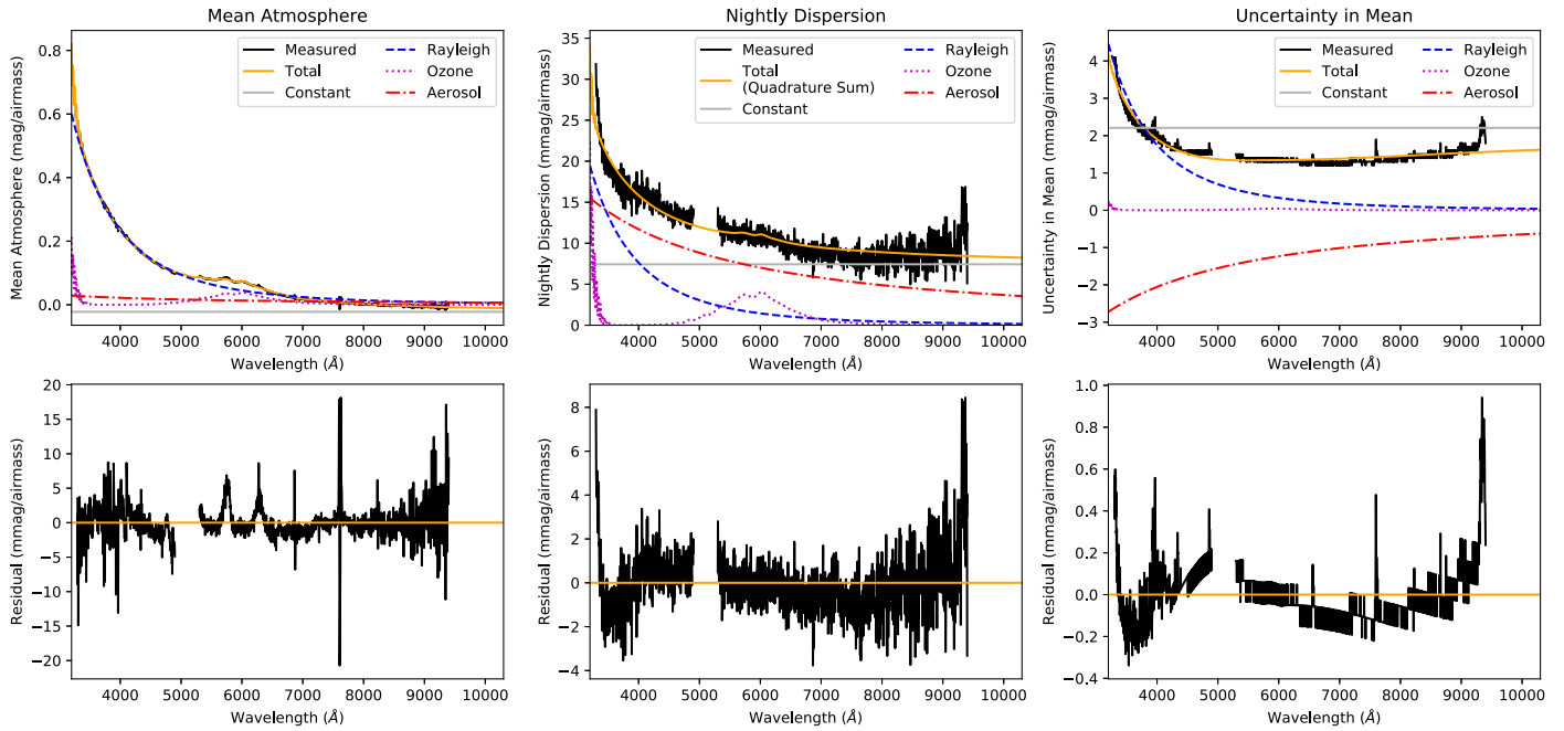
Figure 23. The left column shows the mean atmosphere model ( k_{0,i} from Equation (6)), middle column shows the night-to-night dispersion ( \sigma(k)_i from Equation (6)), and the right panel shows the uncertainty in k_{0,i} (rounded to 0.1 mmag). Upper panels show the measured values with their physical decompositions, while the bottom panels show the residuals after the model is subtracted from the measurements. In the left residual panel, a pair of small discrepancies at the peaks of the ozone Chappuis band is apparent; these are not apparent in the dispersion, suggesting a small error in the Serdyuchenko et al. (2014) ozone template. The residual panels show evidence of a slight convolved-template mismatch at the O_2 A band, but this seems to be static (a glitch visible in the mean, but not in the dispersion). At all other wavelengths, the physical decomposition matches our measured atmosphere to better than a few millimagnitude per airmass.
