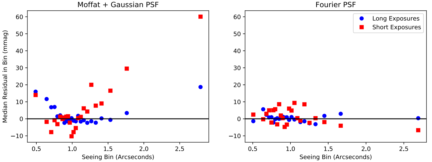
Figure 21. Median residuals vs. seeing in equal-percentile bins for spectra extracted with both PSFs, separated by long and short exposures. The \mathcal{P}_{\text{MG}} PSF (left panel) shows large systematic residuals for both very good and very bad seeing, and these trends are different between long and short exposures. Encouragingly, the \mathcal{P}_{\mathfrak{F}} PSF does better on all fronts, having much smaller residuals (even for very bad seeing), and having similar behavior for both long and short exposures. On the basis of results like this, we chose the \mathcal{P}_{\mathfrak{F}} PSF for our primary results. We note that, for long-exposure standard stars, the two PSFs give consistent calibration to within millimagnitudes, as discussed in the text.
