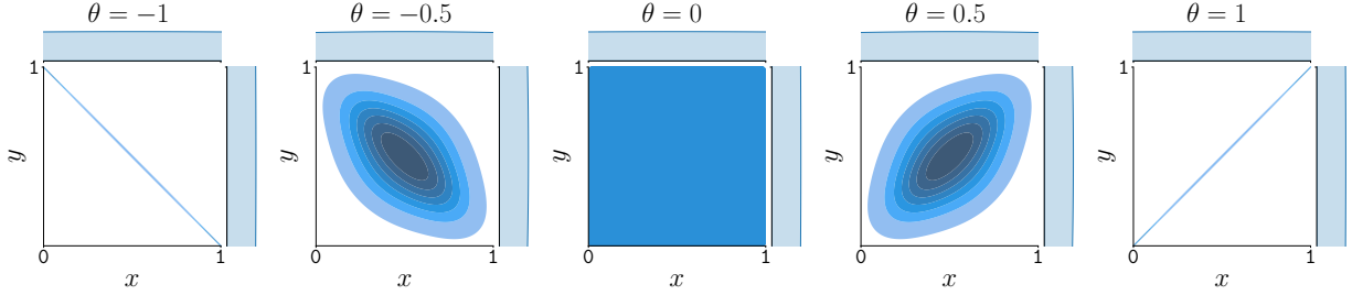
Figure 1 Gaussian copula (i.e., bivariate Gaussian with marginals renormalized to uniform distributions, cf. Appendix A.3) for five different correlation levels, \theta . The shades of blue represent the distribution density (darker means higher).
