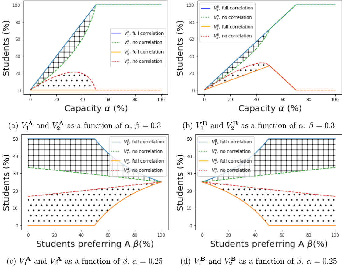
Figure 4: Proportion of students getting their first and second choice with one group, and \alpha_{\mathbf{A}} = \alpha_{\mathbf{B}} = \alpha . The solid blue and orange lines are for the full-correlation case, the dashed green and red ones for the no-correlation case. As the blue and green lines represent the same metric in two different settings, the gap between them is hashed to highlight the welfare increase when switching from one to the other. The same applies to the orange and red lines, where the gap is dotted.
