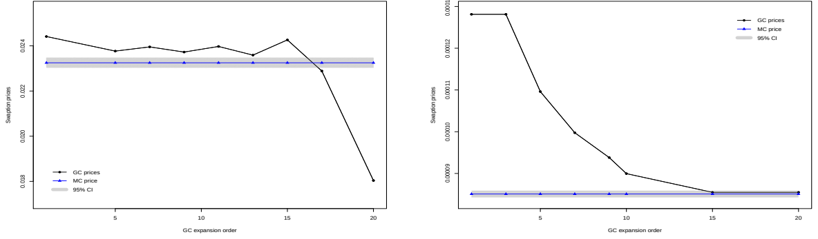
(A) \sigma_r = \sqrt{\text{Var}^S(S_T^{m,n})} = 1.273 \times 10^{-2} , \lambda_{\max}^2 = 1.648 \times 10^{-4} , v_{\max} = 0.5 . Maturity and tenor of the swaption: T = T_m = 5 and T_n - T_m = 5 . (B) 3.203 \times 10^{-4} = \sigma_r \neq \sqrt{\text{Var}^S(S_T^{m,n})} , \lambda_{\max}^2 = 8.097 \times 10^{-7} , v_{\max} = 0.25 . Maturity and tenor of the swaption: T = T_m = 1 and T_n - T_m = 1 .
