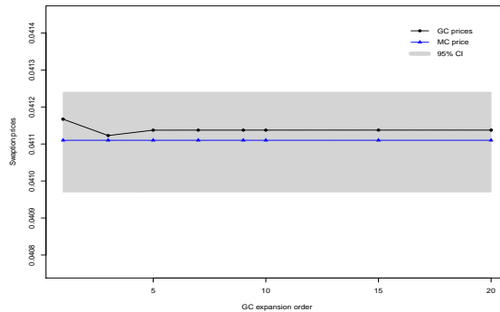
Figure 5: Fast convergence of expanded Gram-Charlier prices with \sigma_r^2 = \text{Var}(S_T^{m,n}) = 4.025 \times 10^{-5} , \lambda_{max} = 1.411 \times 10^{-4} , v_{max} = 0.05 , T_m = 10 , T_n - T_m = 4 , v_0 = 0.015 .
