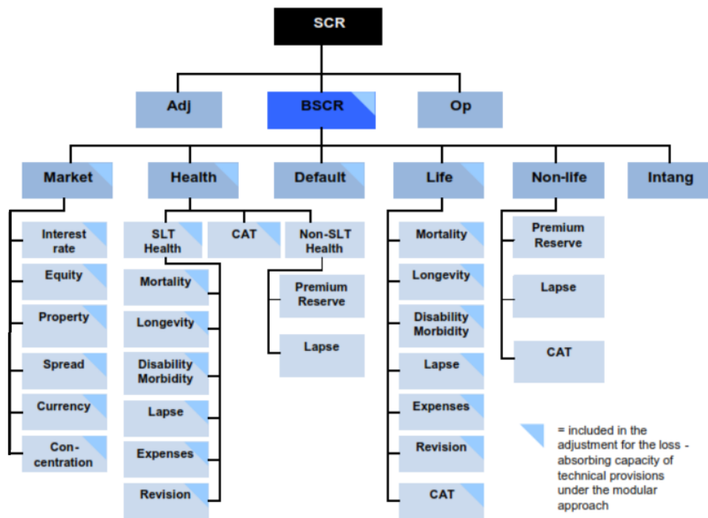
Figure 1: Structure of the Standard Formula in Solvency II.
