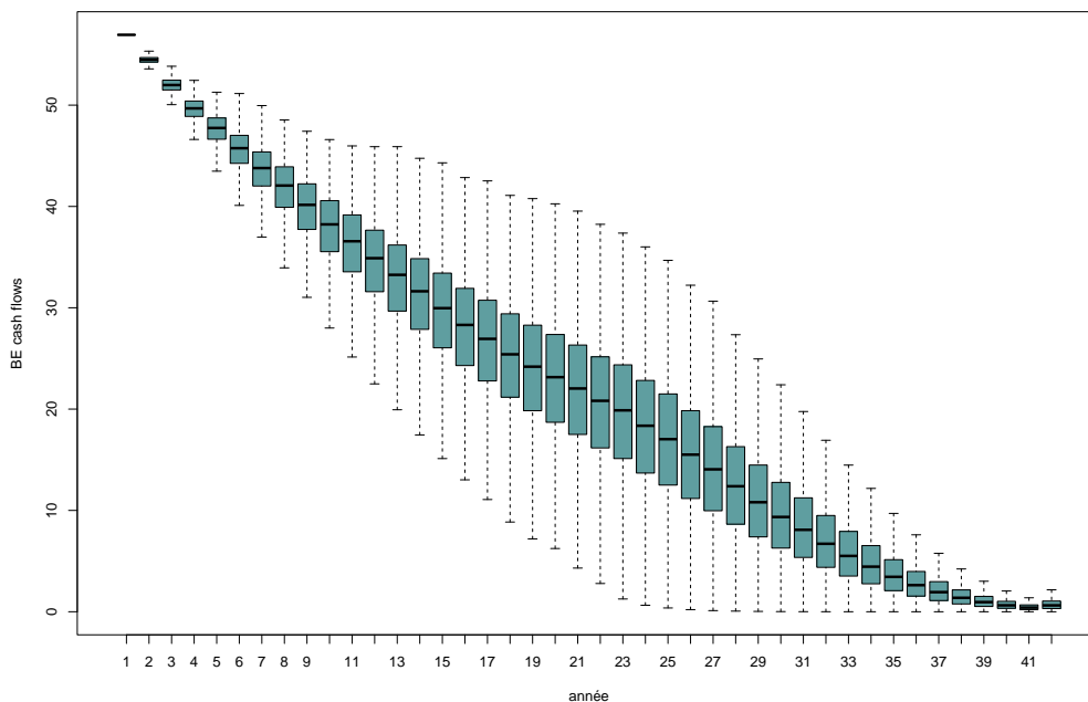
Figure 2: Sequences of BE cash-flows through time. Projection is made on the basis of 3000 interest rates, equity and real estate simulations realized thanks to an ESG calibrated on 12/31/2021.
