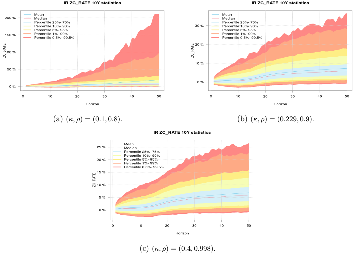
Figure 3: 10Y Zero-Coupon rate quantiles.
