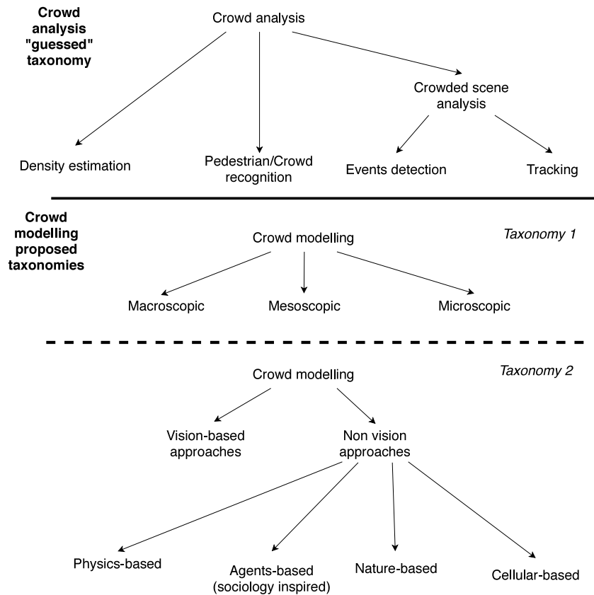
Fig. 1. Taxonomies guessed from Zhan, Monekosso, Remagnino, Velastin, and Xu (2008)'s review.
