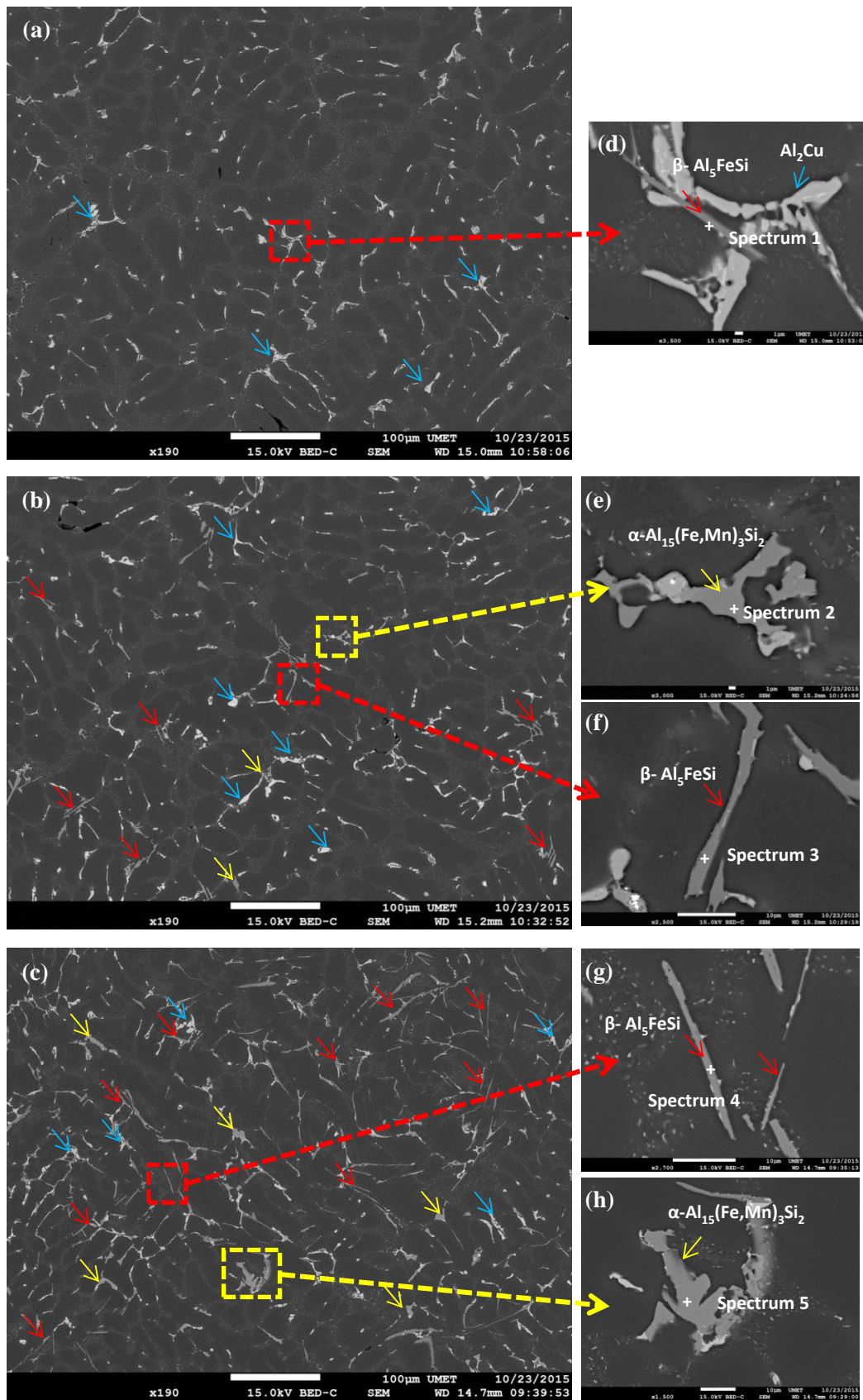
Figure 9 Backscattered electrons SEM micrographs showing the distribution of \alpha -phase \text{Al}_{15}(\text{Fe,Mn})_3\text{Si}_2 (yellow arrow) with a script morphology, \beta -phase \text{Al}_5\text{FeSi} (red arrow) with a needle morphology and \text{Al}_2\text{Cu} phase (blue arrow) in the (a) alloy B, (b) C and (c) D. Points of EDX microanalysis are labeled, and the results are available in Table 5.
