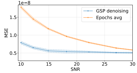
Fig. 2. Evolution of the MSE (avg \pm std) between the true ERP (without noise) and: (blue) the ERP approximation returned by Problem (1) (denoising); (orange) the raw ERP, as a function of the SNR.
