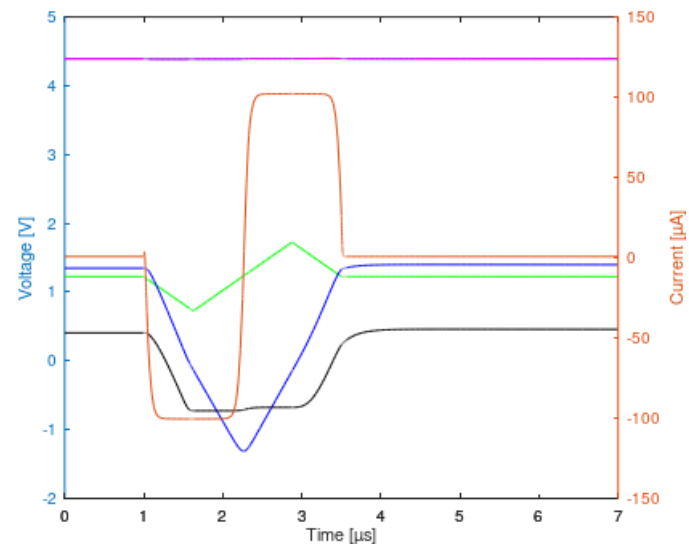
Fig. 17. Plot with different waveforms obtained during SPICE simulation of not propagating SET: VRef voltage (green), OpAmp output (magenta), VCCS output voltage - capacitance of the output stage (blue), OpAmp output transistor base voltage (black), VCCS current (orange).
