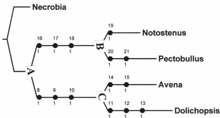
Fig. 22. - Computer generated phylogenetic tree.
