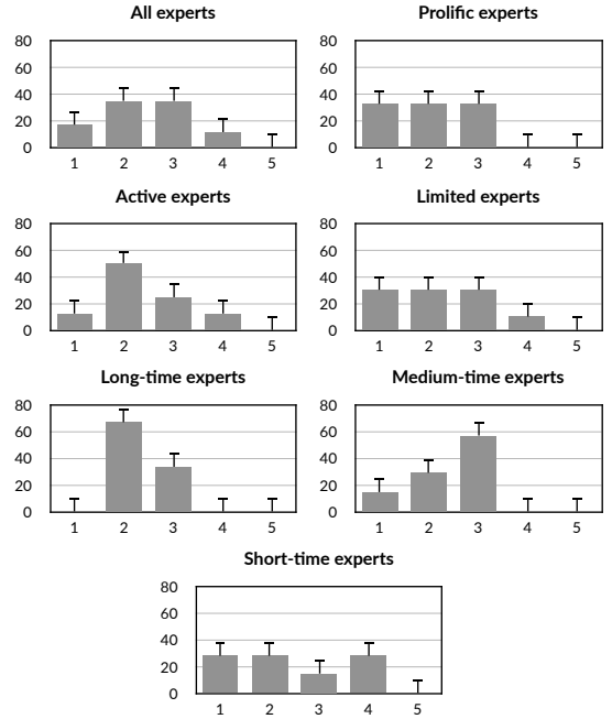
Figure 11: Time-to-insight results.
